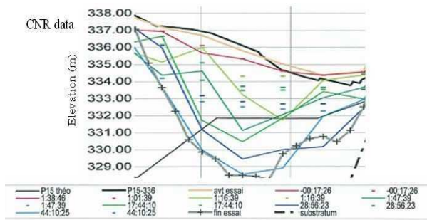
Figure 5. Test Case 17: profile 15 data of the CNR.
