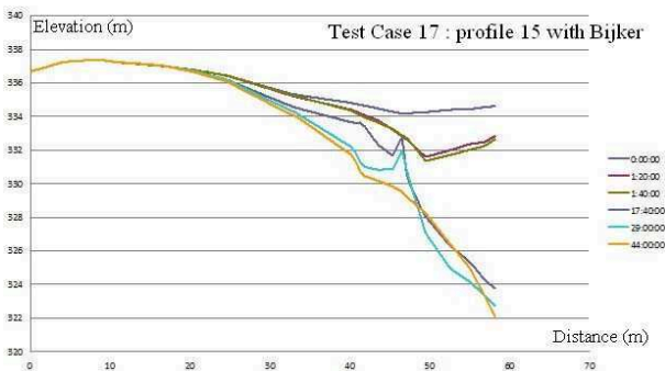
Figure 6. Test Case 17: profile 15 simulated with Bijker formulae.
