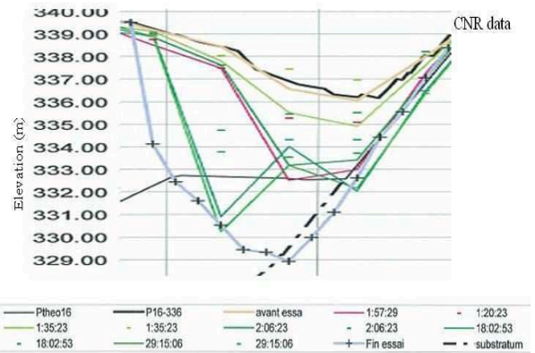
Figure 9. Test Case 17: profile 16 data of the CNR.
