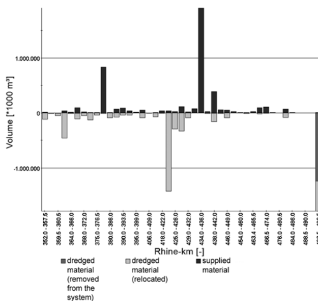
Figure 8. Dredged and supplied sediment volumes between Rhine-km 341 and 502 (for the period 1970-2007). Note: only those river sections are shown where dredging and supply activities occurred. The data is differentiated whether the dredged material is completely removed from the system or re-added to the river at other locations. Note: the data do not include the sediment supply downstream of the barrage at Iffezheim with an average annual volume of 180,000 m 3 .
