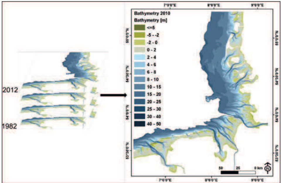
Figure 5: Example for an annual bathymetry (digital terrain model) and layers for spatial and temporal uncertainty.
