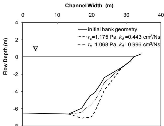
Figure 6 Eroded bank geometry after 10 days
