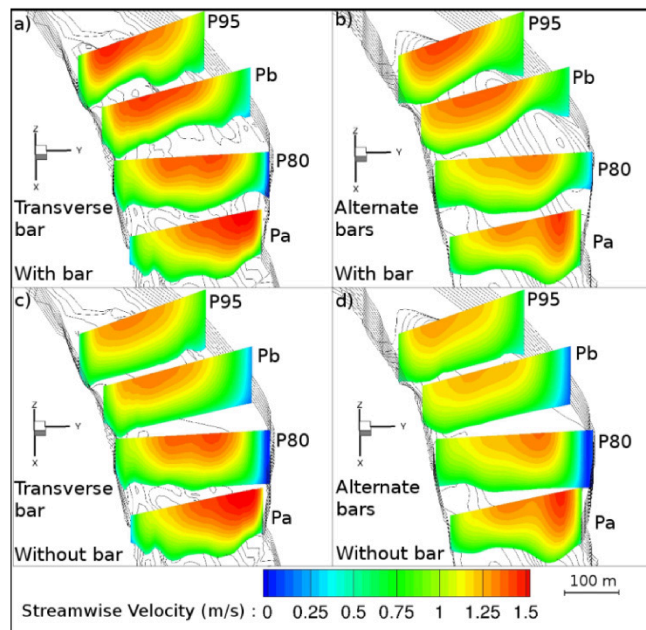
Figure 6. Cross-sectional and vertical distribution of streamwise velocities at 1000 m 3 /s; a) transverse bar configuration, b) alternate bars configuration, c) transverse bar configuration with the bar deleted, d) alternate bars configuration with the bars deleted.
