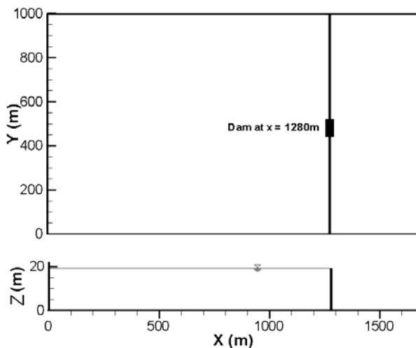
Figure 6. Representation of domain with dam at x=1280 m.
