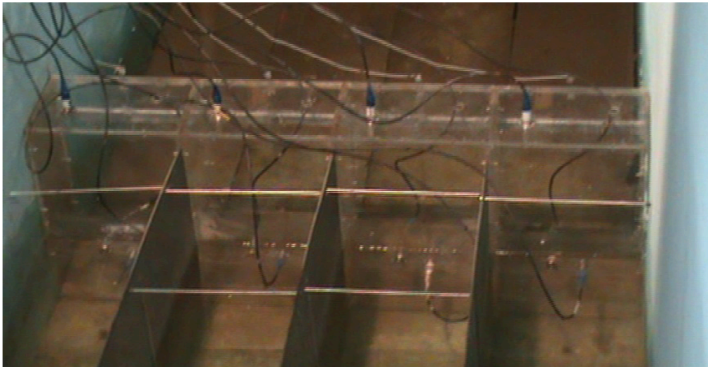
Figure 3. Setup of OWC in wave flume.
