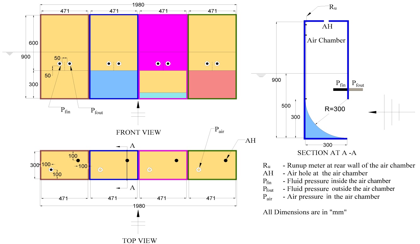
Figure 2. Details of OWC models tested.
