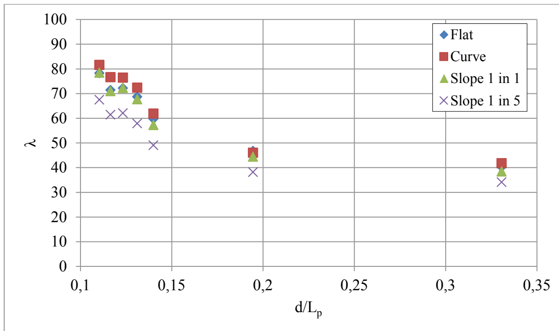
Figure 8. Effect of bottom profile configuration on \lambda with d/L_p ( H_{m0}/d from 0.1010 to 0.1564)
