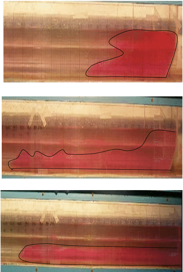
Figure 2: Gravity Current (H=14 cm, Density Difference 0.3%) at three locations (x=50 cm, x=120 cm, x=300 cm).
