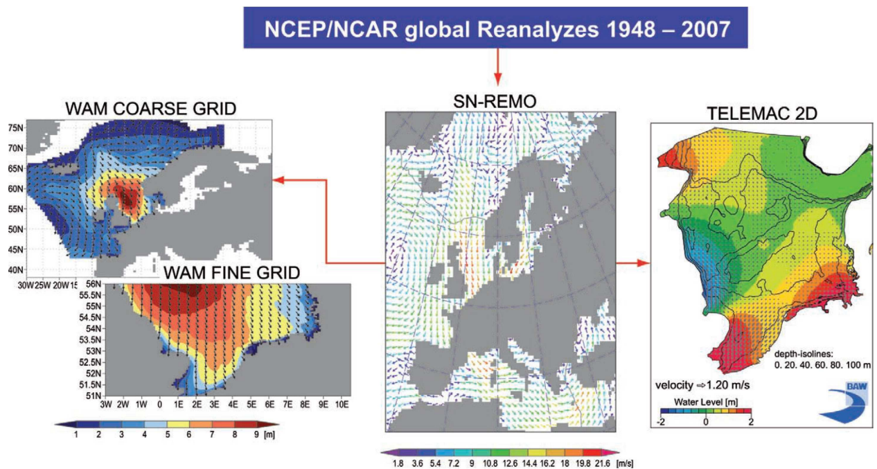
Fig. 1: Layout of the consistent metocean hindcast 1948–2007 for the southern North Sea. From the (middle) regional atmosphere hindcast hourly wind fields were used to force a (right) tide surge and a (left) wave model hindcast. The figure shows an example of consistent metocean conditions obtained from the hindcast for 1200 UTC 21 Feb 1993. (middle) Near-surface (10-m height) marine wind fields ( \text{m s}^{-1} ), and corresponding wind direction obtained from the regional atmospheric reconstruction. (left) Corresponding significant wave height fields (m) and mean wave direction from the coarse and the fine grid wave model hindcast. (right) Tide surge levels (m) from the corresponding tide surge hindcast. After Weisse and Günther (2007).
