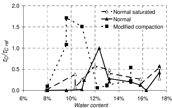
Figure 5 Relative variation of the critical shear stress \tau_c for the P2 soil according to the water content at compaction.
