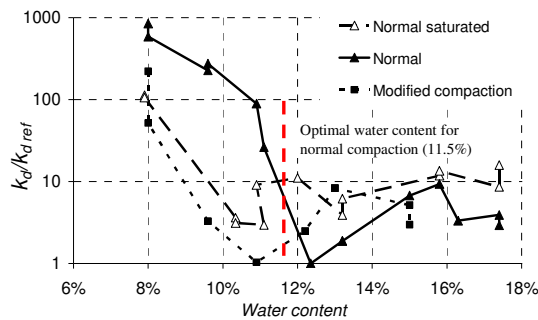
Figure 4 Relative variation of the erosion coefficient k_d for the P2 soil according to the water content at compaction.
