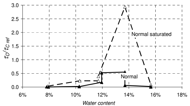
Figure 7 Relative variation of the critical shear stress \tau_c for the P3 soil according to the water content at compaction.
