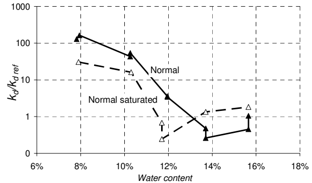
Figure 6 Relative variation of the erosion coefficient k_d for the P3 soil according to the water content at compaction.
