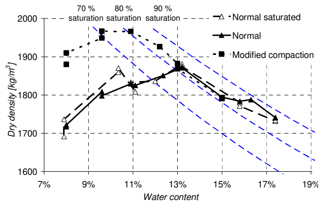
Figure 2 Dry density versus water content at compaction for the P2 soil.
