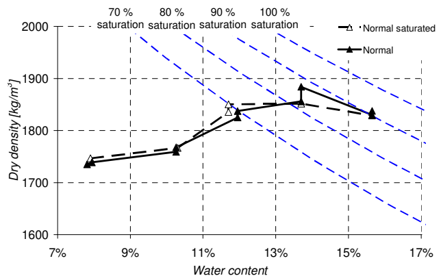
Figure 3 Dry density versus water content at compaction for the P3 soil.
