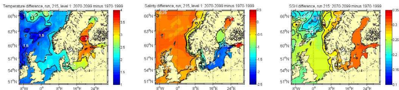
Figure 3: SST Anomalies in °C (left), sea surface salinity (middle) and steric effect in meters (right). Differences are calculated from the difference between the two 30 year periods at the end of the 21th and 20th centuries of the A1B scenario.
