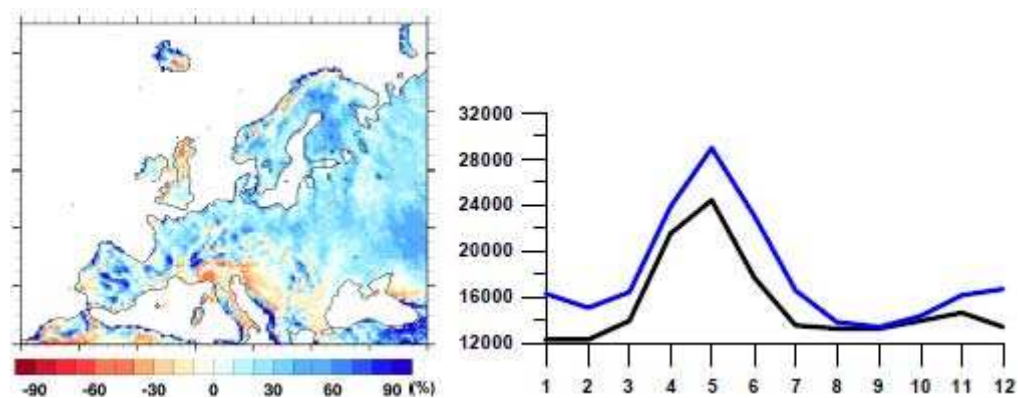
Figure 2: Left: 1970-1999 percentage difference of the simulated precipitation with respect to CRU climatology (Climatic Research Unit, University of East Anglia) (CRU, 2008). Right: Baltic Sea Runoff climatology in m^3 s^{-1} for river observations from GRDC (in black) (Duemenil et al 2000) and simulated (in blue) data.
