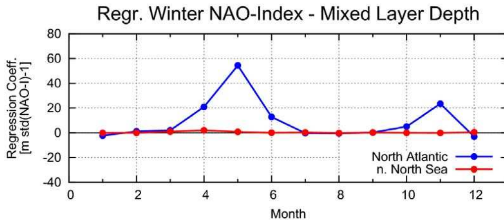
Figure 6: Monthly regression coefficients of winter NAO-Index and MLD for the North Atlantic (blue) and the northern North Sea (red). Analysis of the 20th century control run for the IPCC SRES scenario runs, simulated with the coupled atmosphere-ocean regional circulation model REMO/MPIOM.
