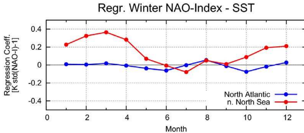
Figure 5: Monthly regression coefficients of winter NAO-Index and SST for the North Atlantic (blue) and the northern North Sea (red). Analysis of the 20th century control run for the IPCC SRES scenario runs, simulated with the coupled atmosphere-ocean regional circulation model REMO/MPIOM.
