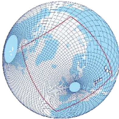
Figure 1: Global ocean domain and domain boundaries of the regional atmospheric model (in red). Please note that not all the grid lines were plotted.
