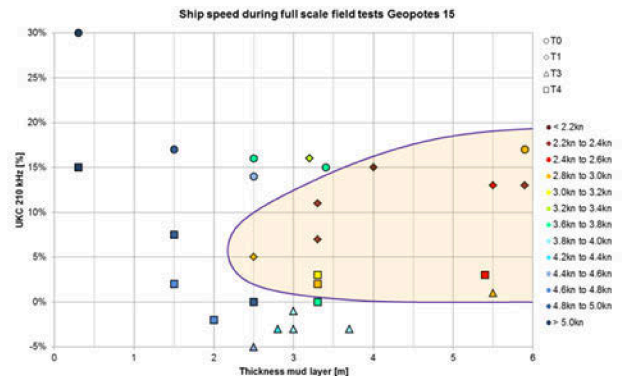
Figure 9. Summarizing graph of the evolution of the speed of the 'Geopotes 15' in function of the sediment layer thickness and the under keel clearance to the top of the fluid mud layer (source FHR).
