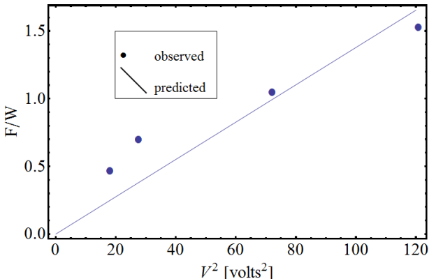
Figure 6. Best fit curve (predicted) showing the linear relation of electromagnetic force to the square of voltage and corresponding experimental data points (observed).
