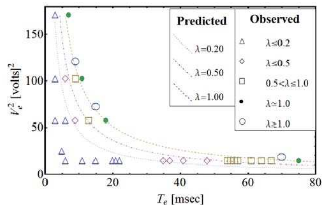
Figure 4. Comparison of different mobility levels as predicted by the theory for various values of \lambda (predicted), with experimentally obtained data points for changing impulse levels (observed) below, at and above critical.
