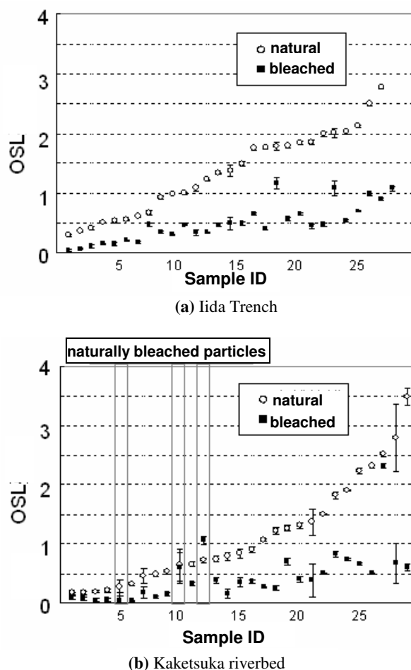
Fig. 8 OSL intensities of sand samples collected at (a) Iida trench and (b) Kaketsuka riverbed
