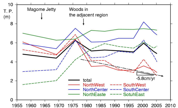
Fig. 5 Temporal variation of mean elevations on Nakatajima Sand Dune
