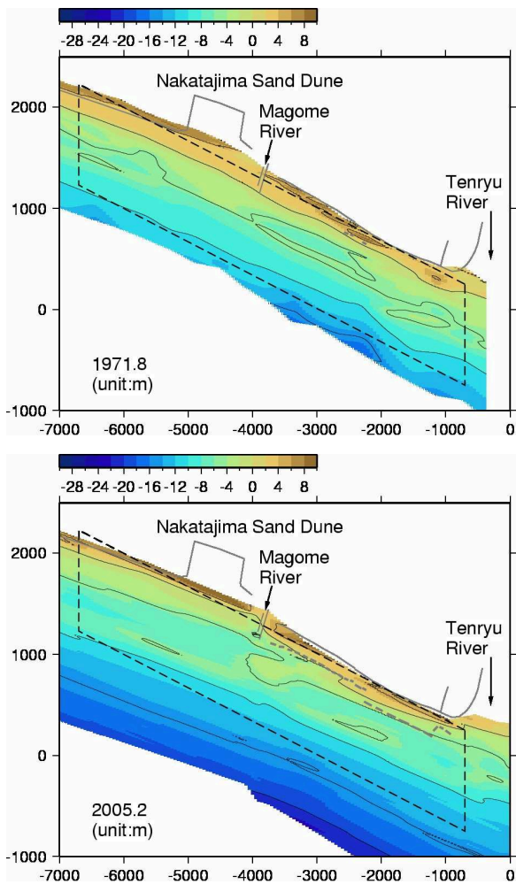
Fig. 2 Nearshore bathymetries of Hamamatsu Coast (1971 and 2005)
