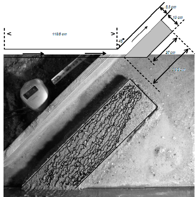
Figure 3. Friedkin experiment. Top: dimensions; sediment block in gray. Bottom: Flow is from the bottom left through the diagonal channel. Block of sediment and bank recognized lines of all time steps drawn in black. Stopwatch and ruler for time and length scale control.
