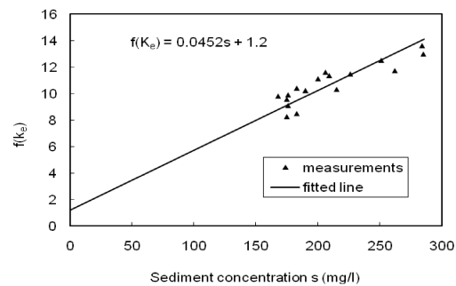
Figure 4. Relationship between f(k_e) and sediment concentrations (based on Eq. 5,
