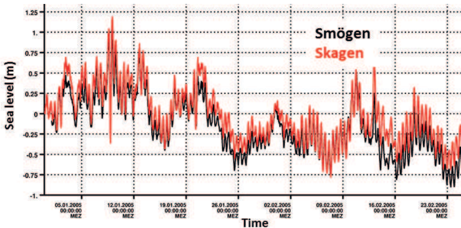
Figure 2: Typical time series at the open boundary.
