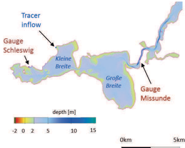
Figure 6: Model bathymetry of the inner Schlei Fjord with inflow position and gauge positions.
