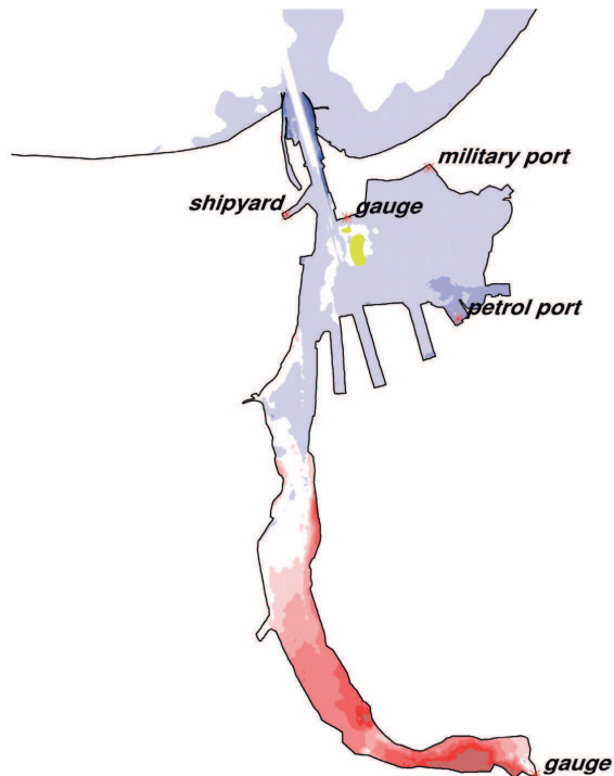
Figure 5: Change in the variability of salinity in the region of the Warnow mouth due to a deepening of the fairway.
