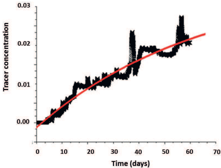
Figure 7: Evaluation of tracer concentration at a station in the inner Schlei Fjord due to entrainment. The markers show the modelled values, the straight line the exponential fitting curve.
