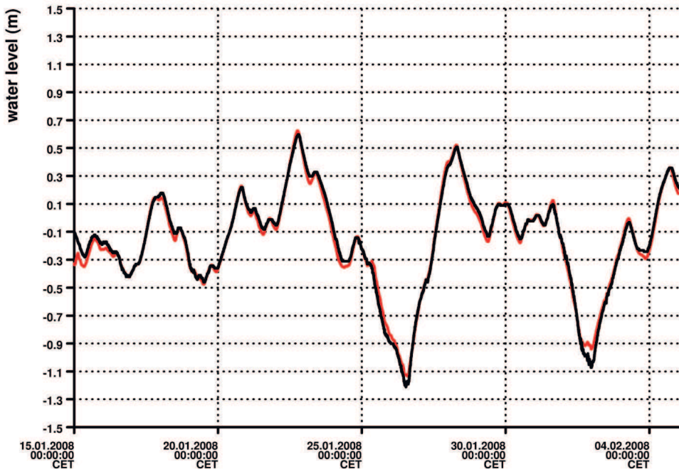
Figure 4: comparison of simulated water level (red curve) with gauge values (black curve) at Schleswig.
