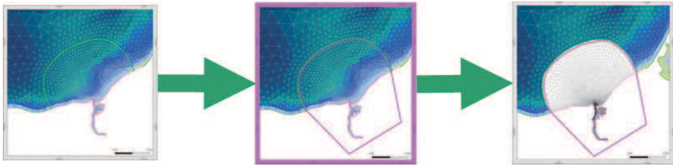
Figure 1: Principle of generation of a regionally refined grid by substitution of an area by an inlay grid.
