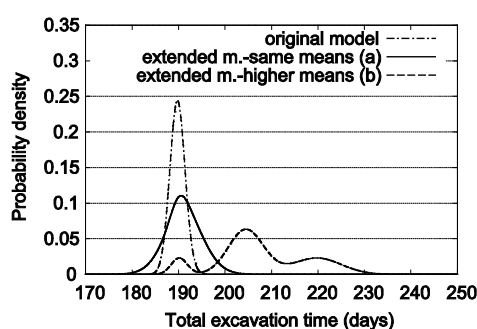
Figure 5. PDF of total time for excavation of Dolsan A tunnel – comparison of models.
