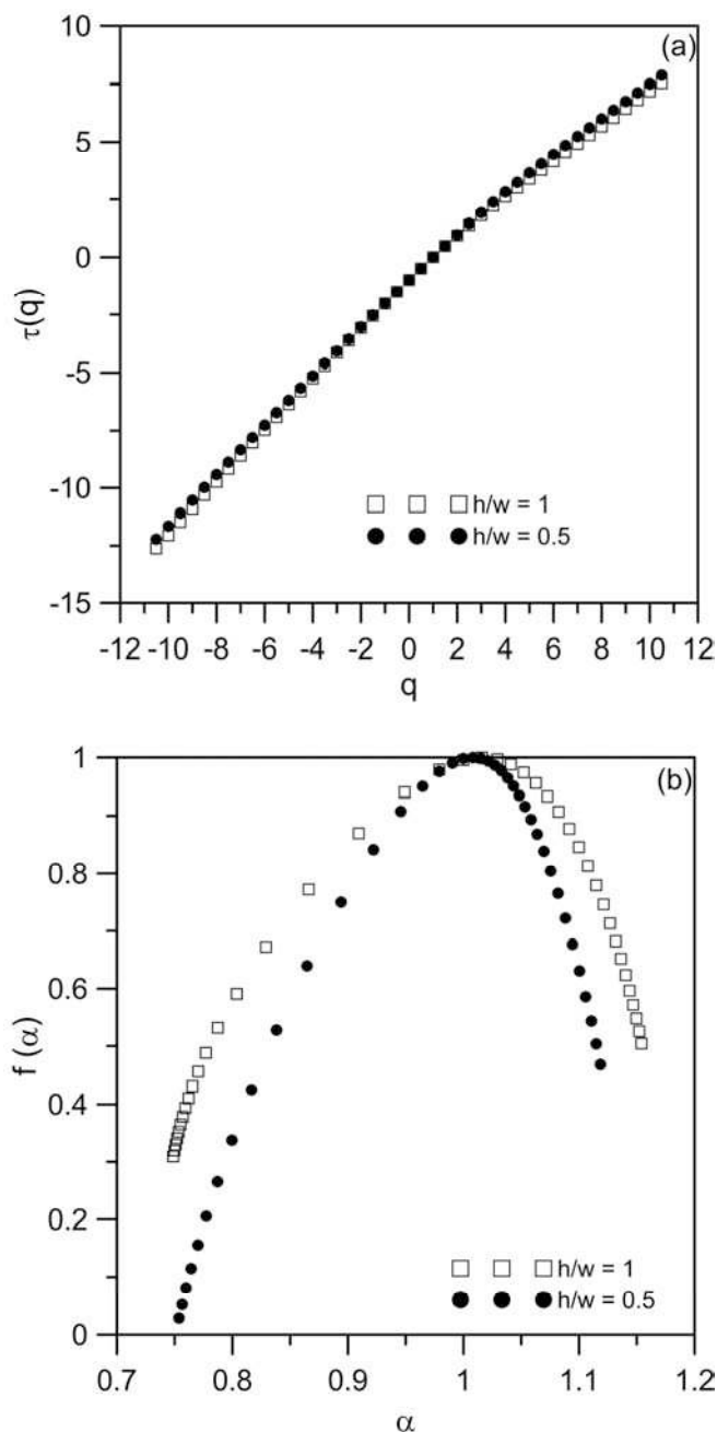
Figure 5. (a) The mass exponent functions \tau(q) and (b) multifractal spectra obtained for the simulated time series in the passive tracer transport for the skimming ( h/w = 1 ) and wake interference ( h/w = 0.5 ) flows.
