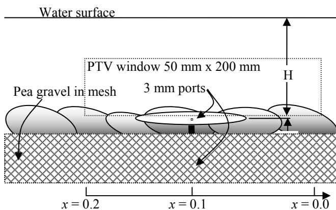
Figure 1. Flume measurement section showing layout and nomenclature. Flow is right to left. Not drawn to scale.
