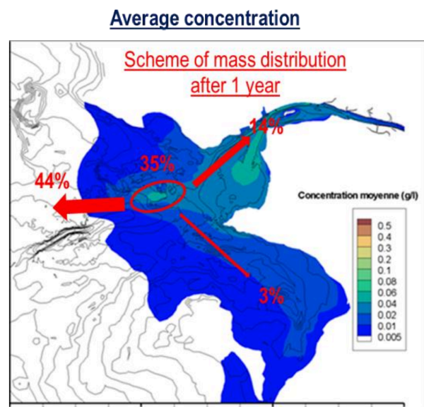
Figure 27. Average concentration of Lambarde sediment dispersion during one year
