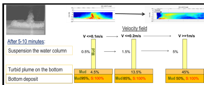
Figure 18. Hypothesis of mass distribution in the near field
