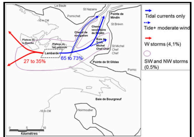
Figure 5. Preliminary study: establishing a first dispersion pattern
