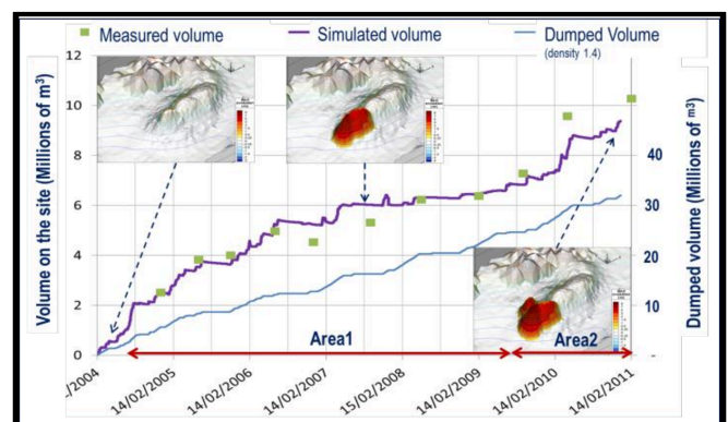
Figure 19. Comparison of the volume on the site
