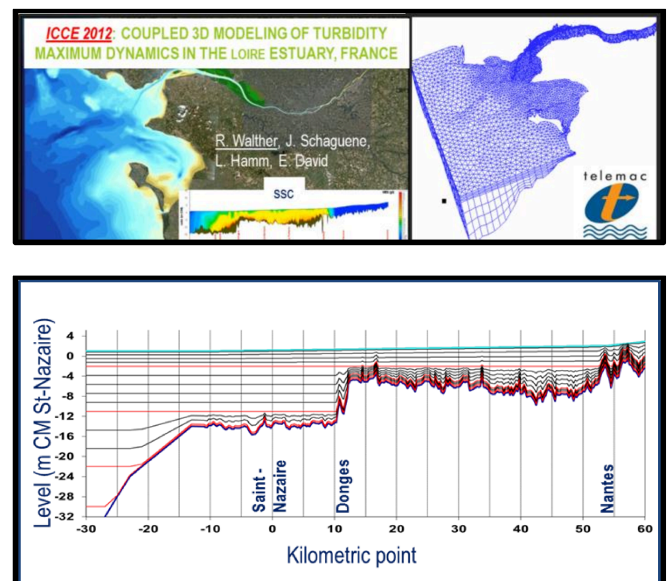
Figure 12. Telemac-3D model of Loire estuary
