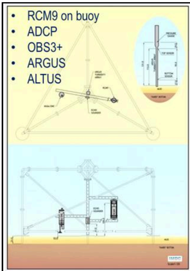
Figure 8. Schem of Lambarde fixed station
