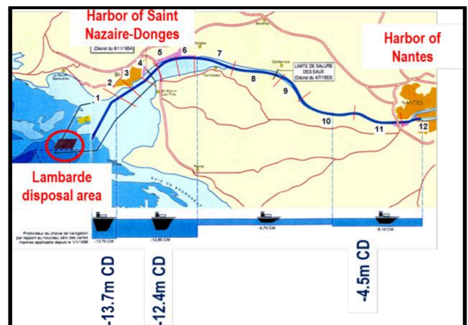
Figure 1. Map of navigation channel and disposal area
