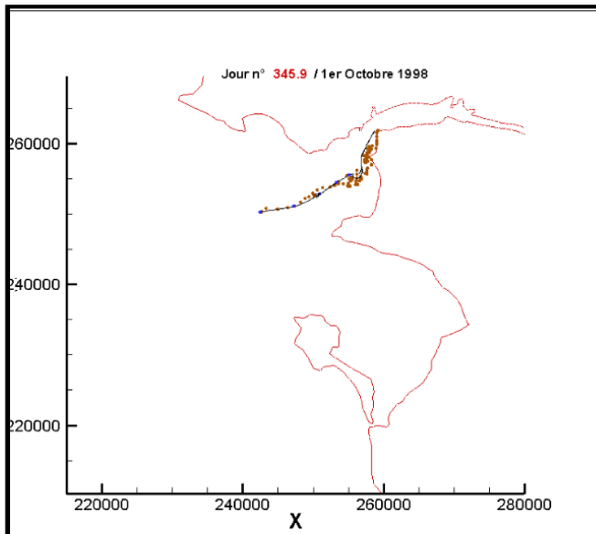
Figure 3. Period 1: Field of particles after 15 days of low flow, low wind (NE ->W) and low waves
