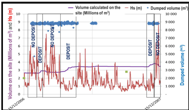
Figure 22. Influence of waves on the stability
