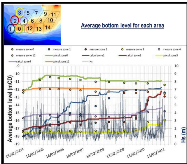
Figure 21. Average bottom level for each area
