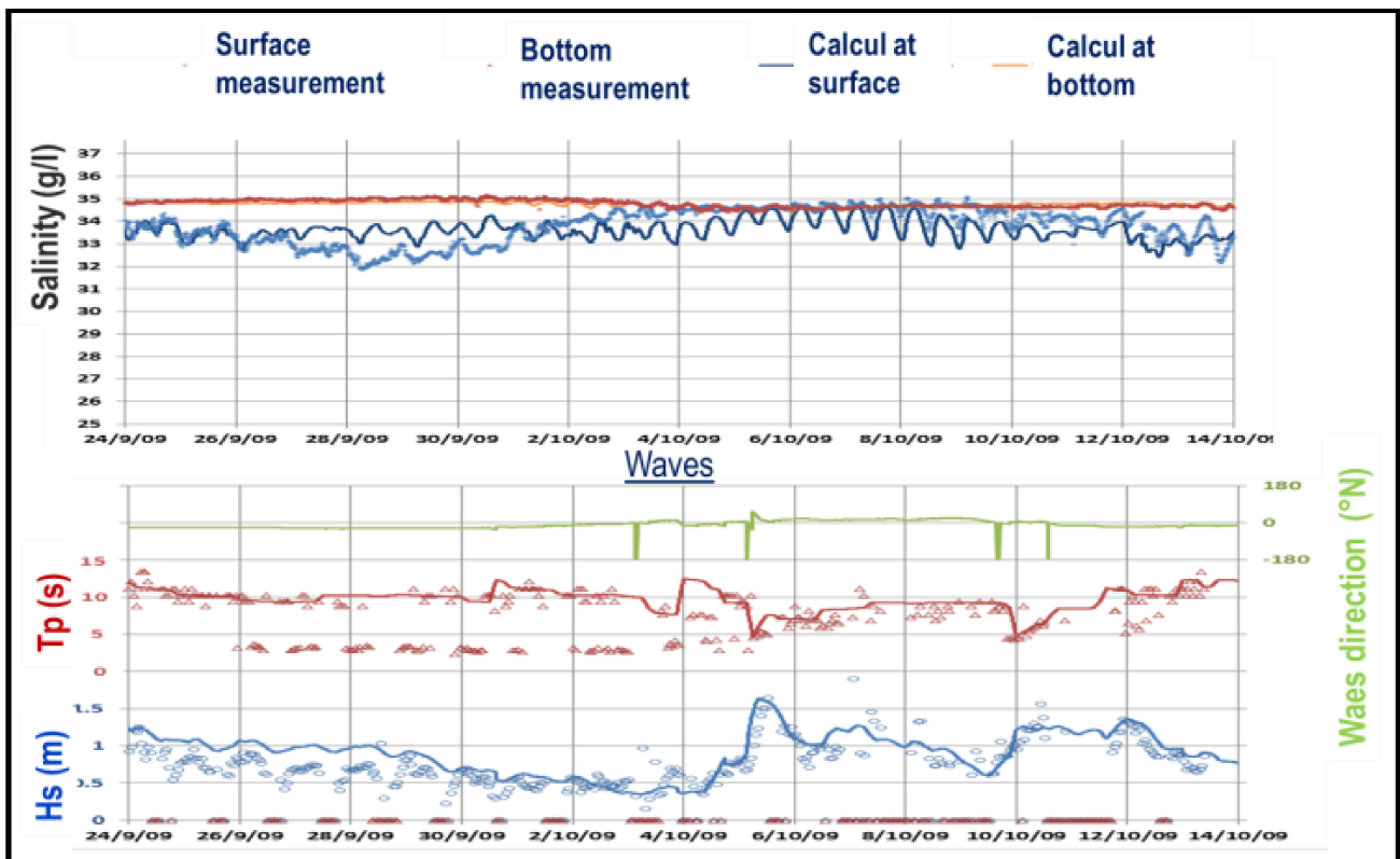
Figure 14. Comparison of salinity at bottom and surface and comparison of waves in amplitude and period
