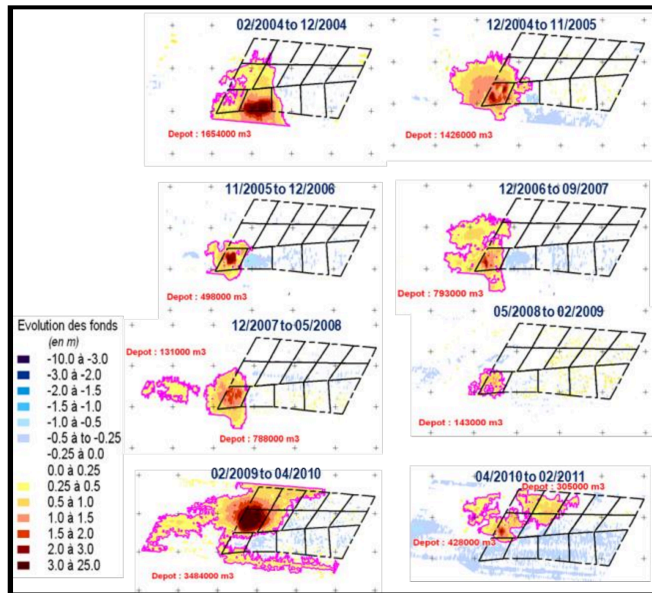
Figure 11. Evolution of Bathymetry
