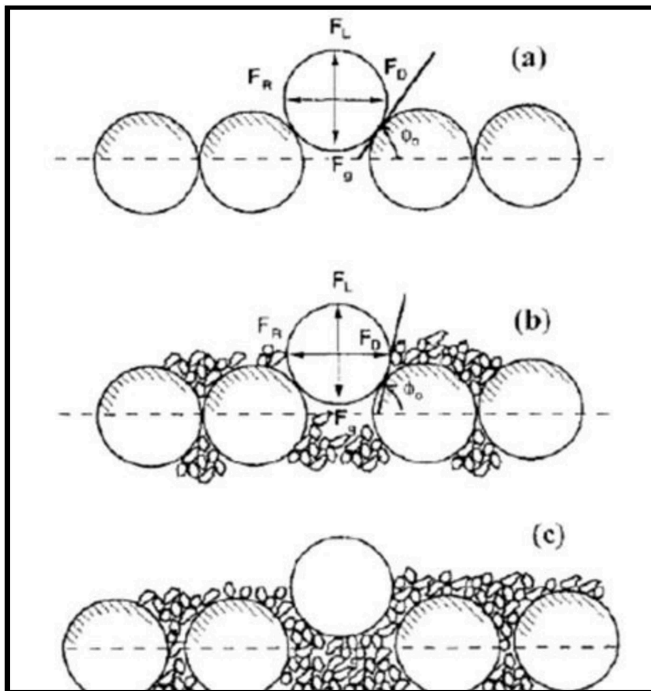
Figure 15. Conceptual diagram showing the implementation mechanism in motion, Panagiotopoulos et al., 1997
