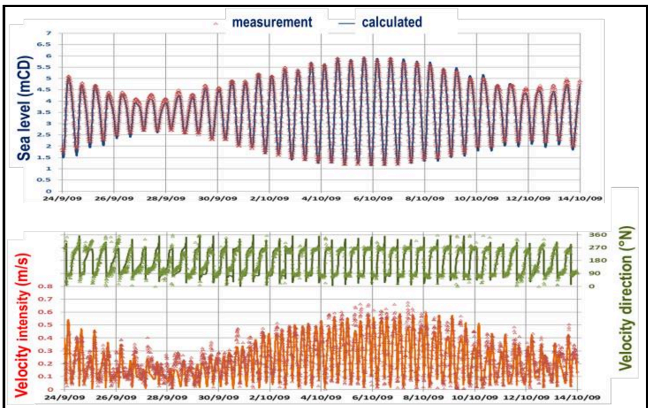
Figure 13. Sea level and velocity comparison
