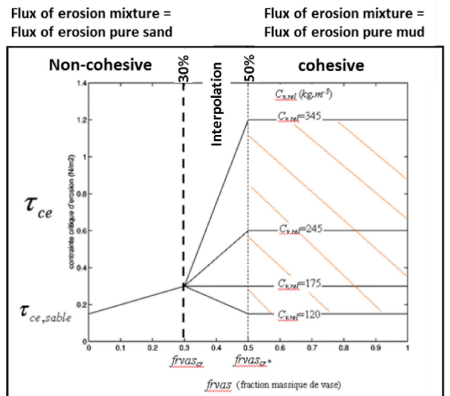
Figure 16. Variation of critical shear stress as a function of mass fraction of mud (Frvas) and relative concentration of mud (Cv,rel), Thesis of B. Waelès 2005 [9].
