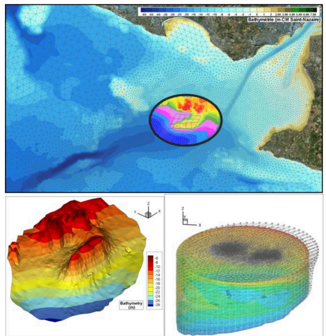
Figure 17. 3D sub-model of stability
