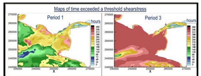
Figure 6. Maps of time exceeded a threshold shear stress for period 1 and 3
