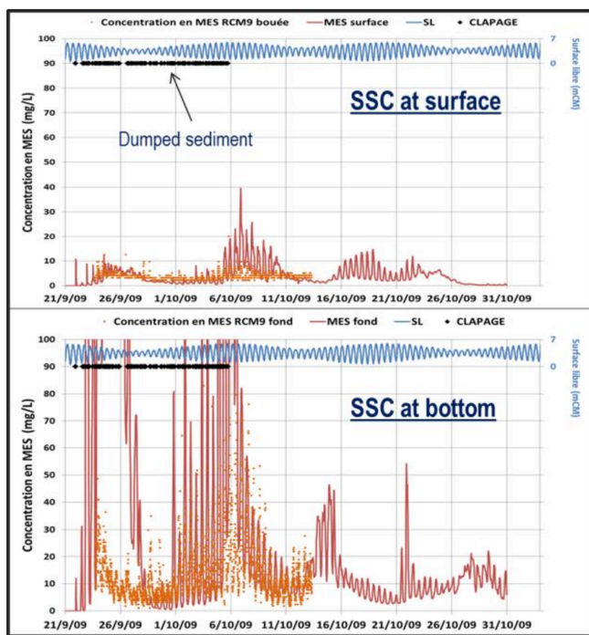
Figure 25. Comparison of suspended concentration at the surface and at the bottom
