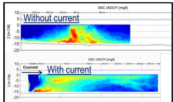
Figure 10. Surface dispersion of the plume under the influence of the current during a Lagrangian protocol measurement.
