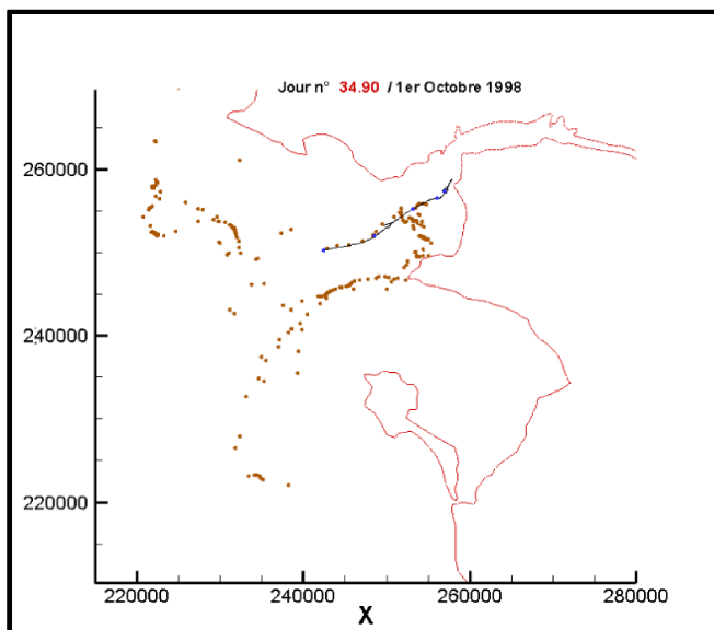
Figure 4. Period 3: Field of particles after 15 days of mean -> low flow, strong wind (W ->NW), mean -> strong waves
