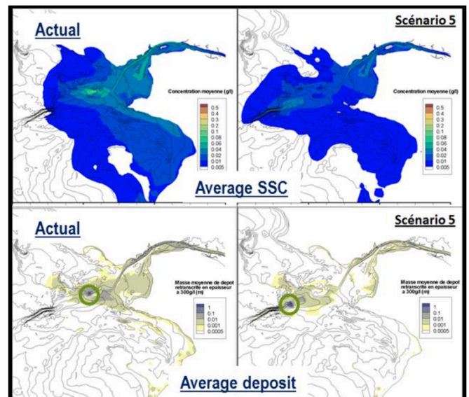
Figure 30. Comparison of dispersion between actual situation and scenario 5
