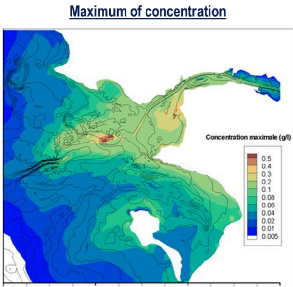
Figure 28. Maximum concentration of Lambarde sediment dispersion during one year
