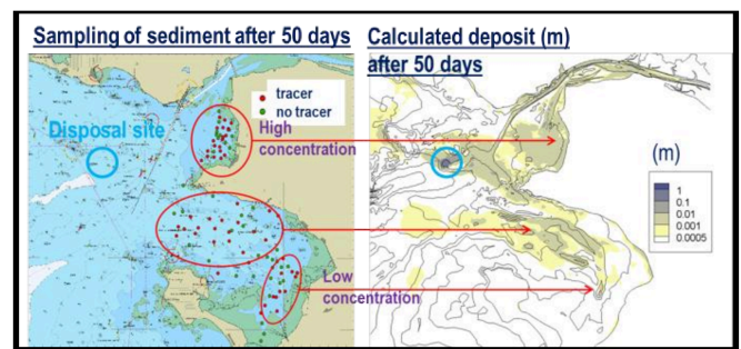
Figure 26. Comparison of tracer measurement and deposit during 1 April-21 May
