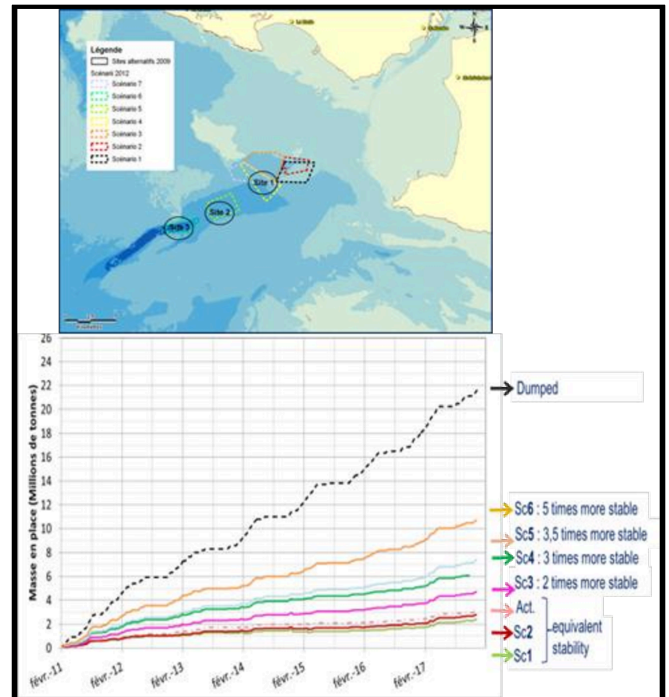
Figure 29. Comparison of stability for 6 scenarii
