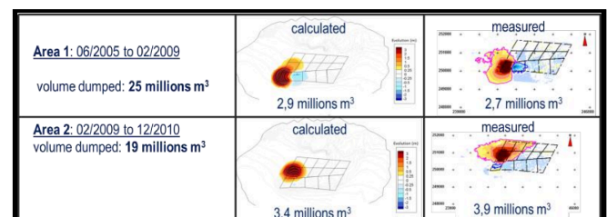
Figure 20. Bathymetry evolution
