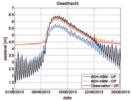
Figure 13: Water levels during Elbe flood at station Geesthacht-UP. Additionally model results at station Geesthacht-OP are shown.
