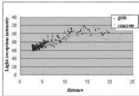
Figure 4. Relationship between distance and light reception intensity
