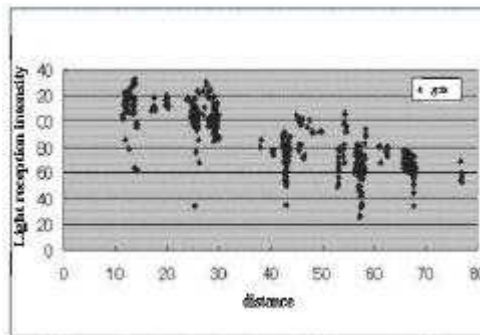
Figure 5. Relationship between distance and light reception intensity (grits and concrete)
