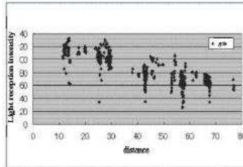
Figure 6. Relationship between distance and light reception intensity (vegetation)
