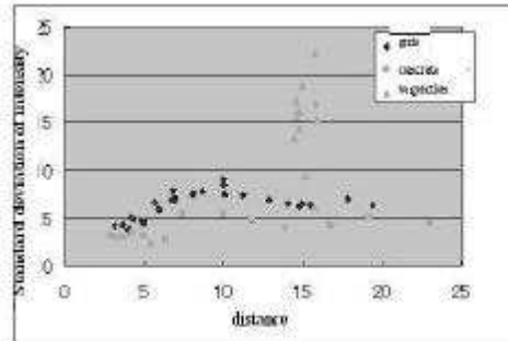
Figure 7. Relationship between distance and standard deviation of light reception intensity (grits, concrete, vegetation)
