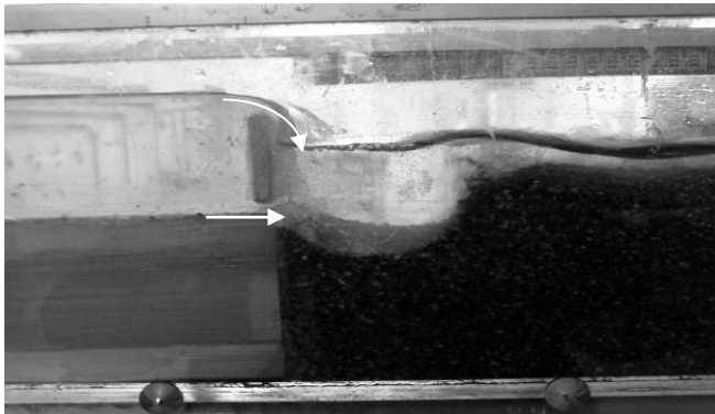
Figure 9 Scouring downstream of combined flow over the weir and under the gate
