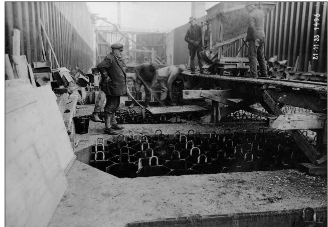
Bild 3: Herstellung des Sohlpflasters Figure 3: Execution of the pavement at the base of the lock
