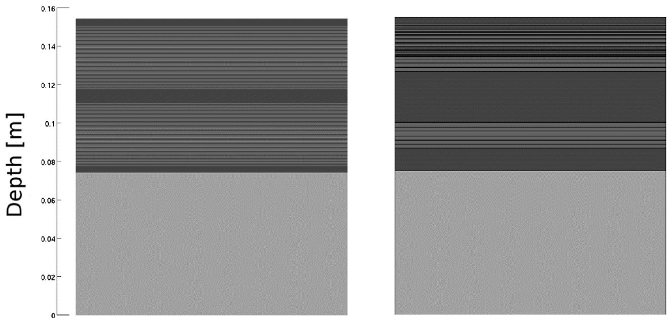
Figure 6. Results from simulation of depositional area after two neap spring cycles. Brighter layers contain a higher fraction of sand. Left picture shows a simulation with a maximum number of layers to store all information. The right picture shows a simulation with a maximum number of layers of 50. Merging of layers has taken place.
