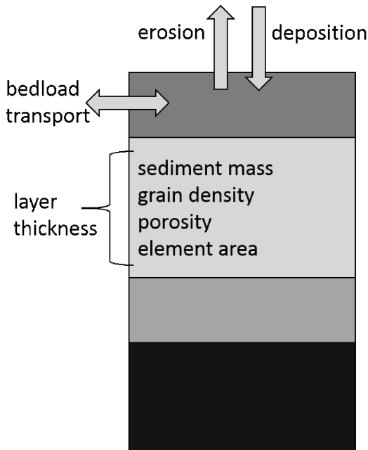
Figure 5. Mass fluxes and stored layer information for calculation of soil evolution.
