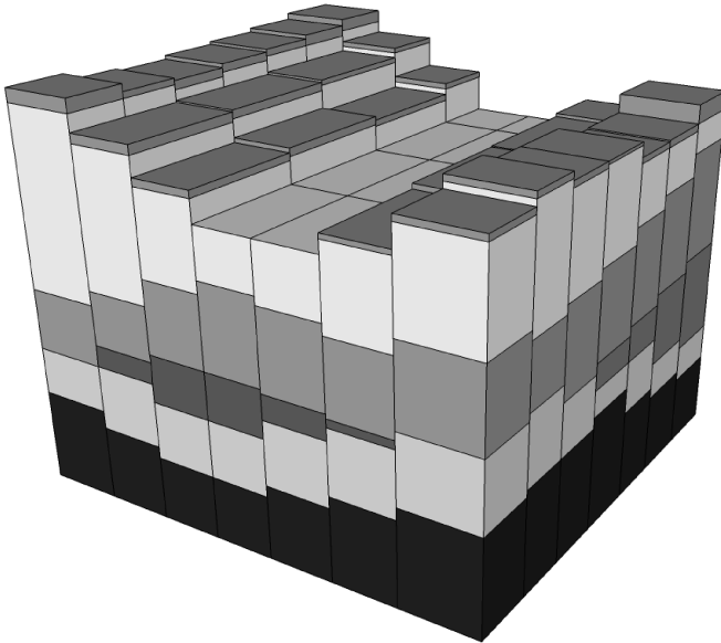
Figure 2. Schematic view of a soil in the model presented here. Brighter colors indicate a higher fraction of sands. The soil can be structured in each grid element with the number of layers that are necessary to describe the vertical differences in sediment distribution.
