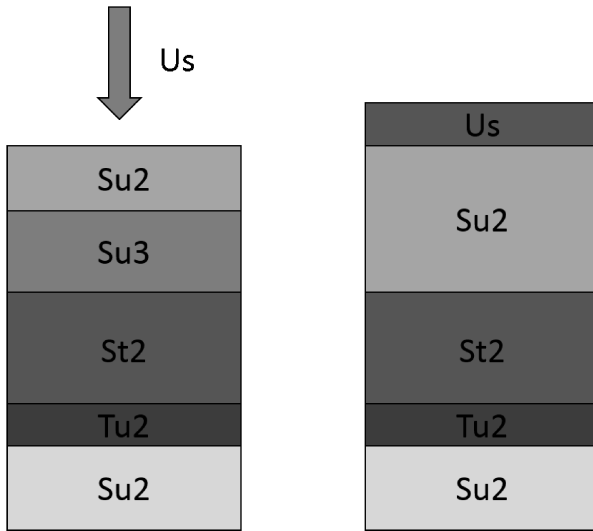
Figure 4. Concept for merging layers when maximum number of layers is reached. The two adjacent layers with the most similarity in sediment distribution in the soil column are merged.
