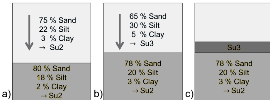
Figure 3. Formation of a new layer: a) Deposition of sediments that differs only slightly from the sediment in the top layer (Su2 = soil texture poor silty sand); b) Deposition occurred in existing layer; Sediment distribution of the depositional flux differs enough from the sediment in the top layer (Su3 = medium silty sand); c) Deposition occurred in new layer.
