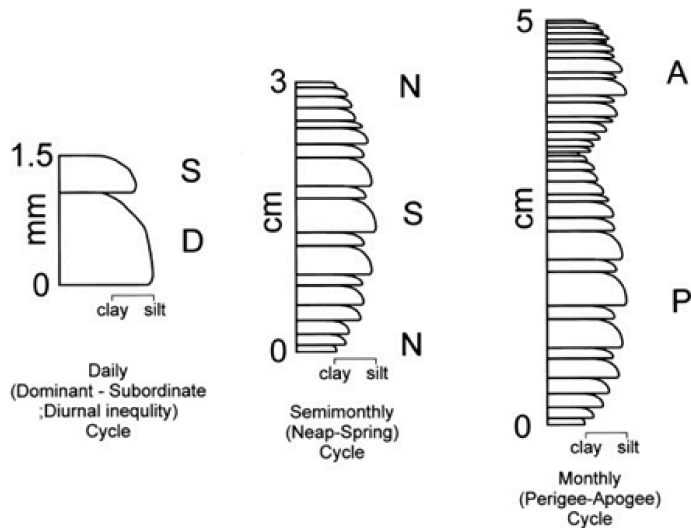
Figure 1. A Schematic principle of the formation of rhythmites and the influence of different periods of the tidal cycle on layer thickness and composition (Choi, 2000).
