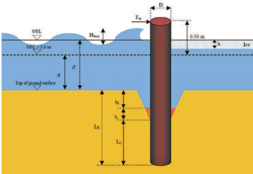
Fig. 8: Sketch for definition of parameters used in the recommendations (WEICHBRODT, 2008)
