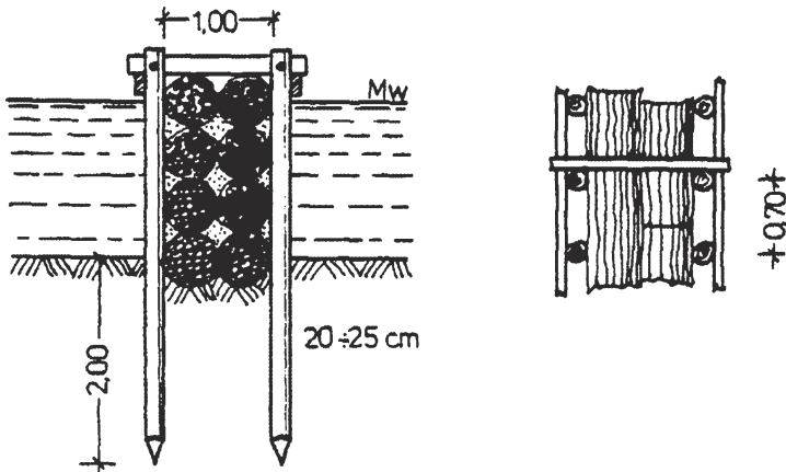
Fig. 6: Wooden groyne construction at the Baltic coast near Warnemünde, 1895 (TRITT and ALTEMEIER, 1987; after FÜLSCHER, 1905)
