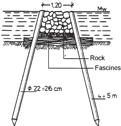
Fig. 7: Wooden groyne construction at the Baltic coast, 1897 (TRITT and ALTEMEIER, 1987; after FÜLSCHER, 1905)
