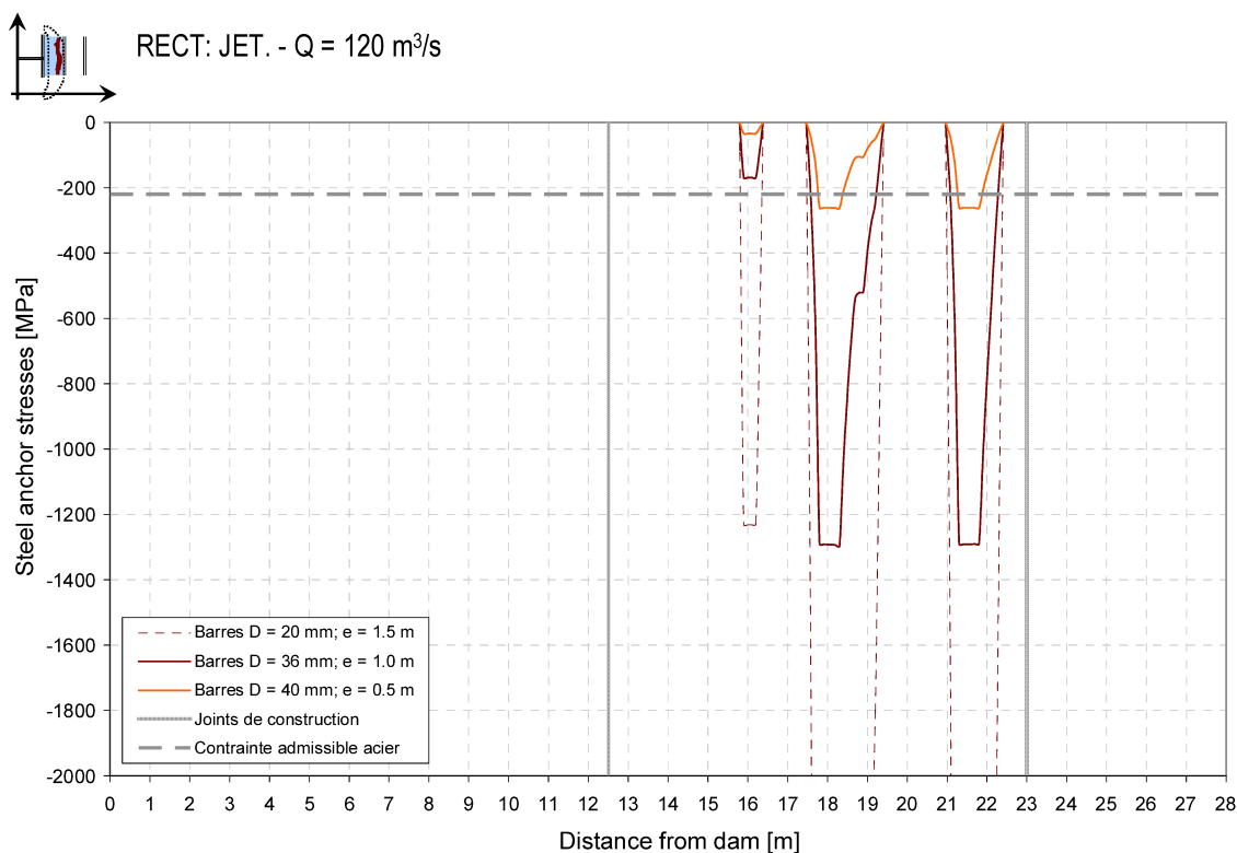
Fig. 9 Steel anchor stresses induced by the 100-year flood
