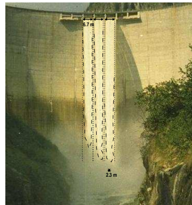
Fig. 6 Shape of jet impacting onto the concrete apron of the plunge pool.
