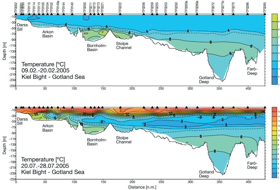
Fig. 3: Horizontal-vertical sections of temperature as in Fig. 2 as recorded during Baltic monitoring cruises (see Fig. 1) in winter (top) and in summer (bottom)
