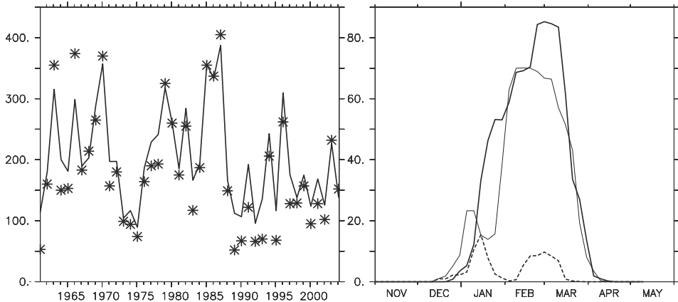
Fig. 9: Yearly maximum ice extent ( 10^3 \text{ km}^2 ) of the Baltic Sea (left panel); the bold line indicates the simulated ice cover and star symbols show the estimates by SEINÄ and PALOSUO (1996). Relative model ice extent (%) in the south-western Baltic (right panel); bold, thin, and dotted lines correspond to the winters 1962/63, 1995/96, and 2002/03
