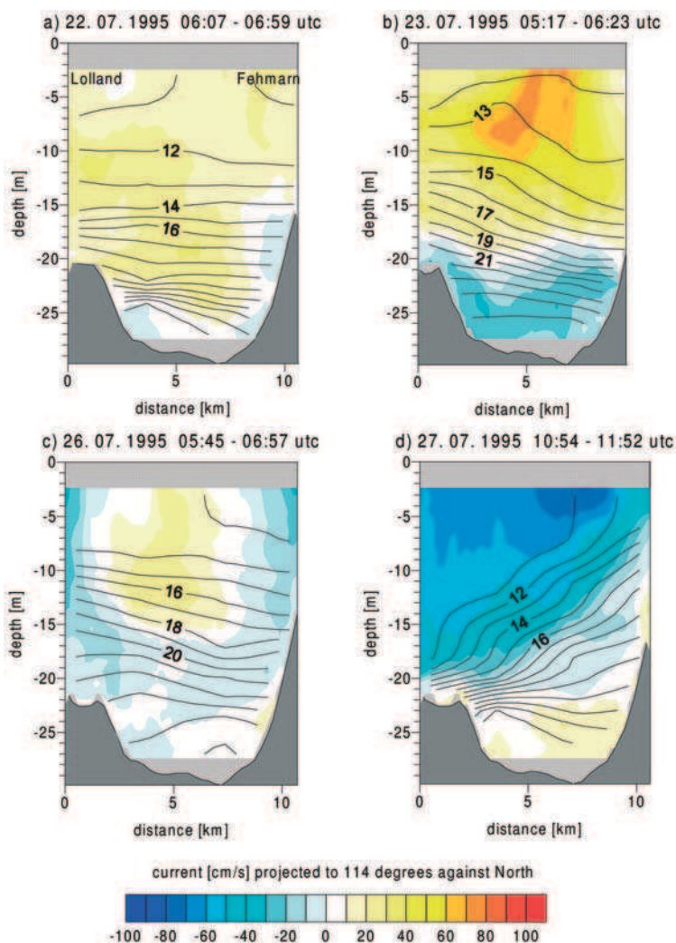
Fig. 7: Four snapshots of salinity stratification (contours) and flow (colours) through the Fehmarn Belt during summer stratification. The shape of the isohalines indicates the geostrophically adjusted status of the currents. The speed ranges from +80 to -80 cm/s, for inflow and outflow, respectively
