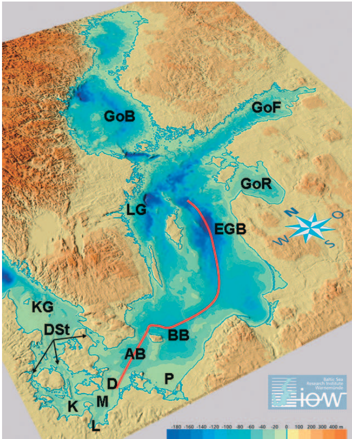
Fig. 1: Topographic map of the Baltic Sea (SEIFERT et al., 2001): Kattegat (KG), Danish Straits (DSt), Kiel Bight (K), Lübeck Bight (L), Mecklenburg Bight (M), Darss Sill (D), Pomeranian Bight (P), Arkona Basin (AB), Bornholm Basin (BB), Eastern Gotland Basin (EGB), Landsort gauge (LG), Gulf of Riga (GoR), Gulf of Finland (GoF), and Gulf of Bothia (GoB). The bold red line indicates the ship track for the records shown in Figs. 2 and 3
