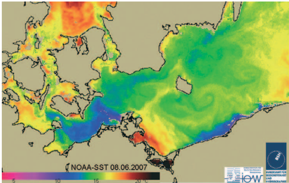
Fig. 5: Satellite image of the south-western Baltic in June 2007. The blue areas indicate cold upwelled water
