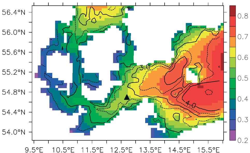
Fig. 4: Mean significant wave height (colours, in meters) and maximum waves (contours) in the period 1990–1999 simulated with an adaptation of a parametric wave model (SCHWAB et al., 1984) with ERA-40 wind forcing (UPPALA et al., 2005). The triangle shows the position of the GKSS wave rider buoy used to validate the model results
