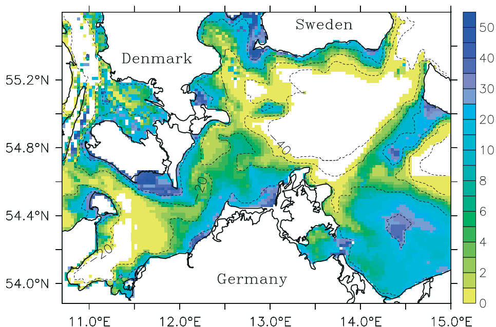
Fig. 10: Modelled frequency of occurrence (%) of fluff erosion in the period Dec. 1992 till Oct. 1993. Broken lines indicate the water depth in 10 m steps
