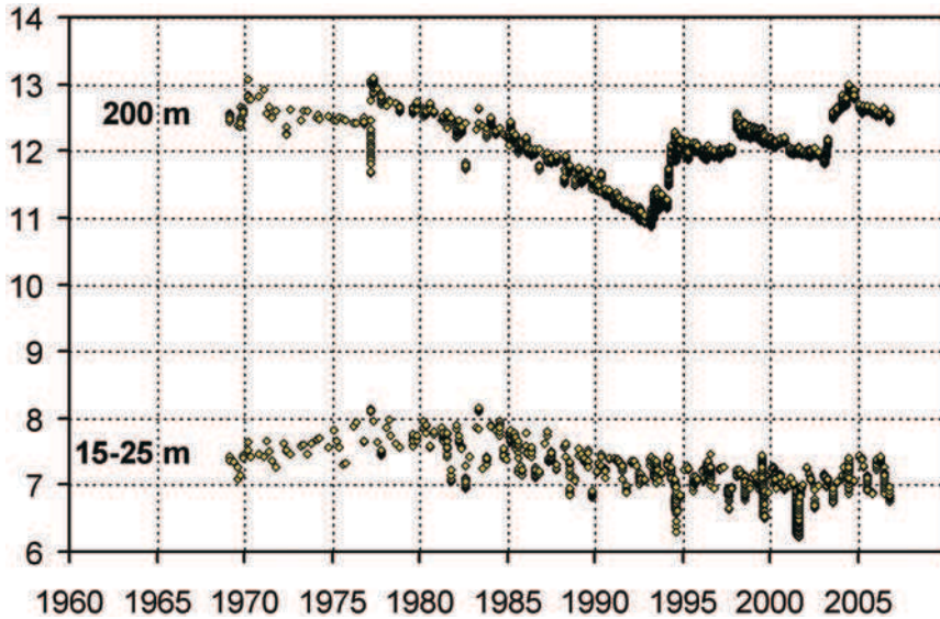
Fig. 8: Time series of salinity in the deep water and near the surface at a station in the central Baltic. The data are taken from the data base of the IOW
