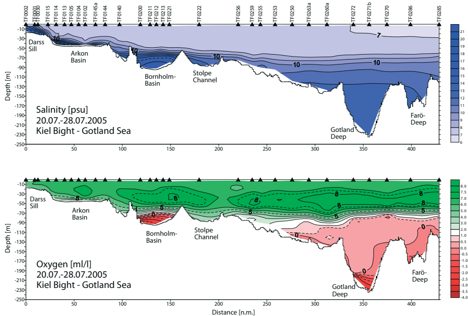
Fig. 2: Horizontal-vertical sections of salinity (top) and oxygen (bottom) as recorded during a Baltic monitoring cruise in 2005 (see Fig. 1). Negative oxygen is used to indicate hydrogen sulphide
