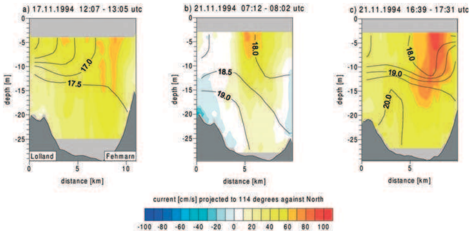
Fig. 6: Three snapshots of salinity stratification (contours) and flow (colours) through the Fehmarn Belt during autumn conditions. The flows show basically an inflow, but the flow pattern is structured and varies over a range of almost 1 m/s
