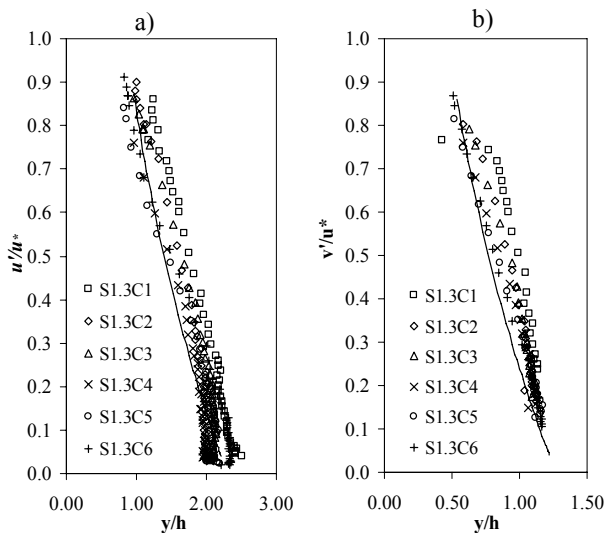
Figure 12. Vertical distribution of turbulence intensities components: a) longitudinal and b) vertical.
