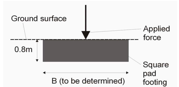
Figure 5. The pad foundation on sand
