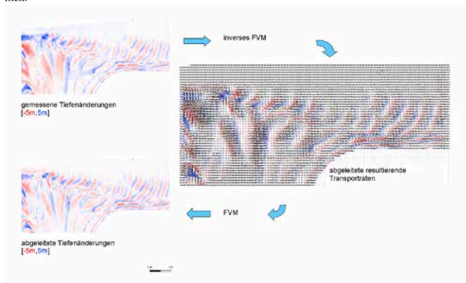
Abb. 26: Inverse Finite-Volumen-Approximation
