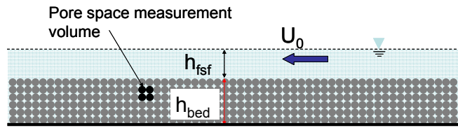
Figure 1. Schematic of the permeable bed model. The channel cross-section dimensions are: width=0.35 m and height=0.60 m. The pore space measurement volume is marked; this was located at 1.68 m downstream from the inlet section and (10 cm underneath the top of the spheres).
