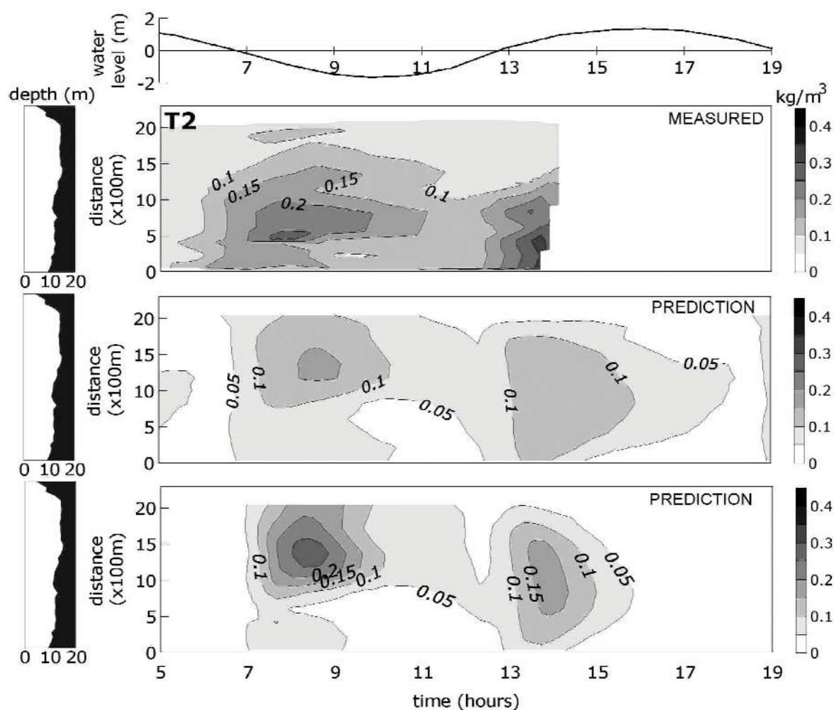
Fig. 11: Measured (upper) vs. computed (BIJKER: middle, VAN RIJN: lower) variation in suspended sediment concentration at cross-section T2 (Suedererpiep) dataset 3 (September 5, 2000)
