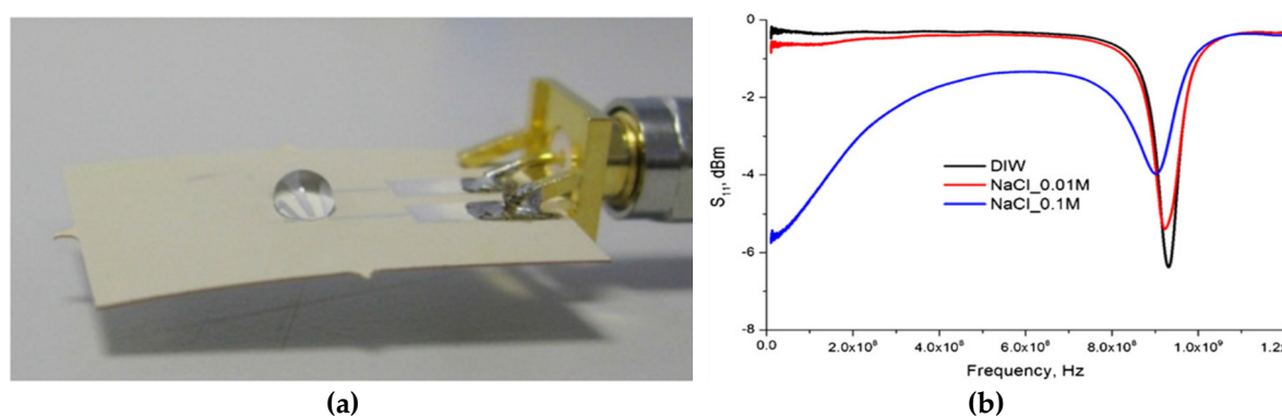
Figure 9. (a) Microwave flexible sensor with 20 \mu\text{L} of water sample placed the silver IDEs and (b) its output sensing response comparing deionized water (DIW), and 0.01 and 0.1M of NaCl. Reproduced with permission from [49] © 2020 IOP Publishing Ltd.
