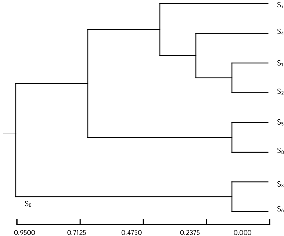
Fig. 1. UPGMA Dendrogram based on Nei's (1972) genetic distance summarizing the data on differentiation among 8 isolates of S. rolfsii
