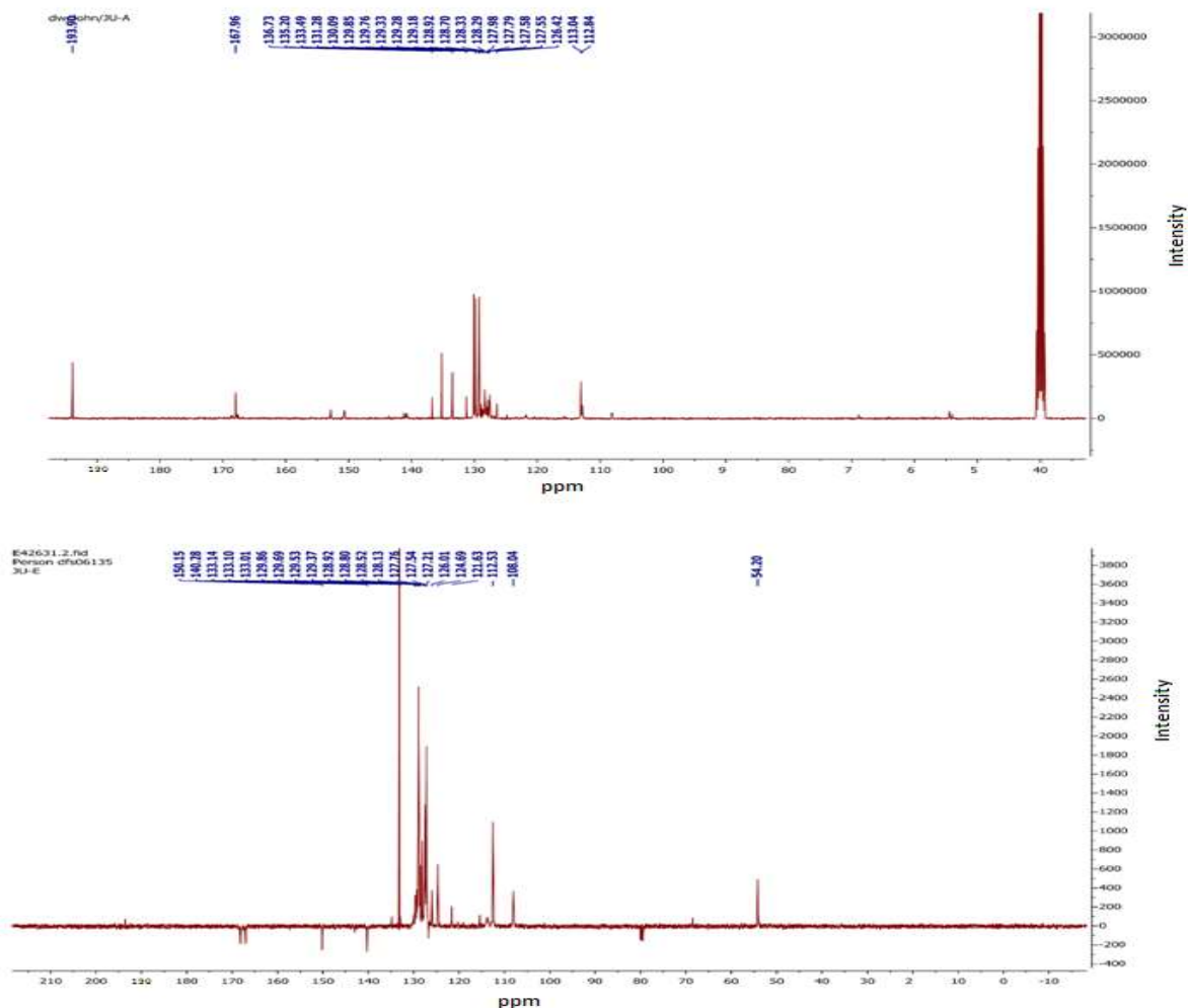
Fig. 4: ^{13}\text{C} -NMR spectra for PTBS and [Ni(PTBS)]
