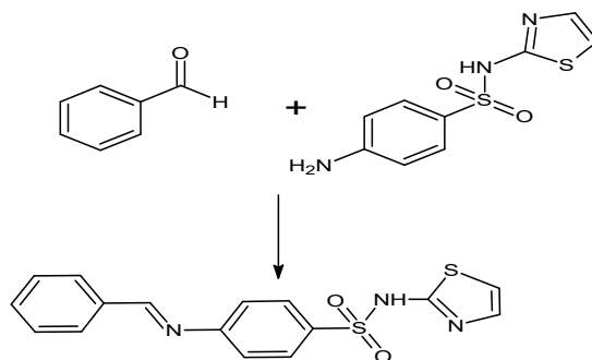
Scheme 1: Synthesis of 4-[(E)-phenylmethylidene]amino}-N-(1,3-thiazol-2-yl)benzenesulfonamide Schiff base ligand (PTBS)
