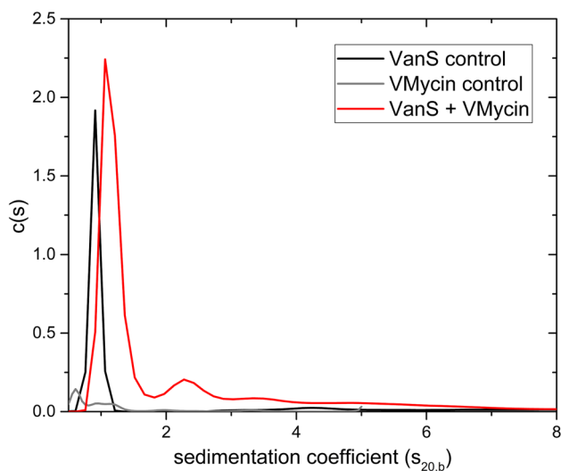
Fig. 7 Sedimentation coefficient concentration distribution, c(s) vs s profile for intact VanS (5.4 \mu M) (black line) in HGN buffer (containing 20% glycerol) pH ~ 7.9, I=0.1 , at 20.0 °C. The rotor speed was 40,000 rpm. The profile for 12.8 \mu M vancomycin is shown (grey line). VanS and vancomycin is shown by the red line under the same conditions. Reproduced with permission from Phillips-Jones et al. (2017a) Sci Rep 7:46,180
