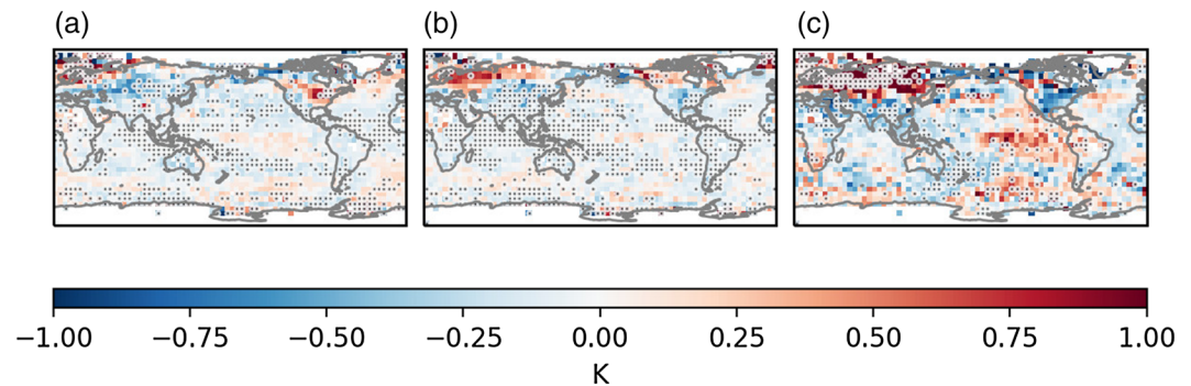
Figure 19. Surface temperature anomalies for the two Northern Hemisphere winters (December-January-February) following the volcanic eruptions for (a) GC31-LL, (b) GC31-MM, and (c) HadCRUT4. All major volcanic eruptions across all members have been averaged to bring out the robust response. Anomalies significant at the p = 0.05 level using a two-sided t test are stippled. The model fields have been masked where there are no observations in HadCRUT4.
