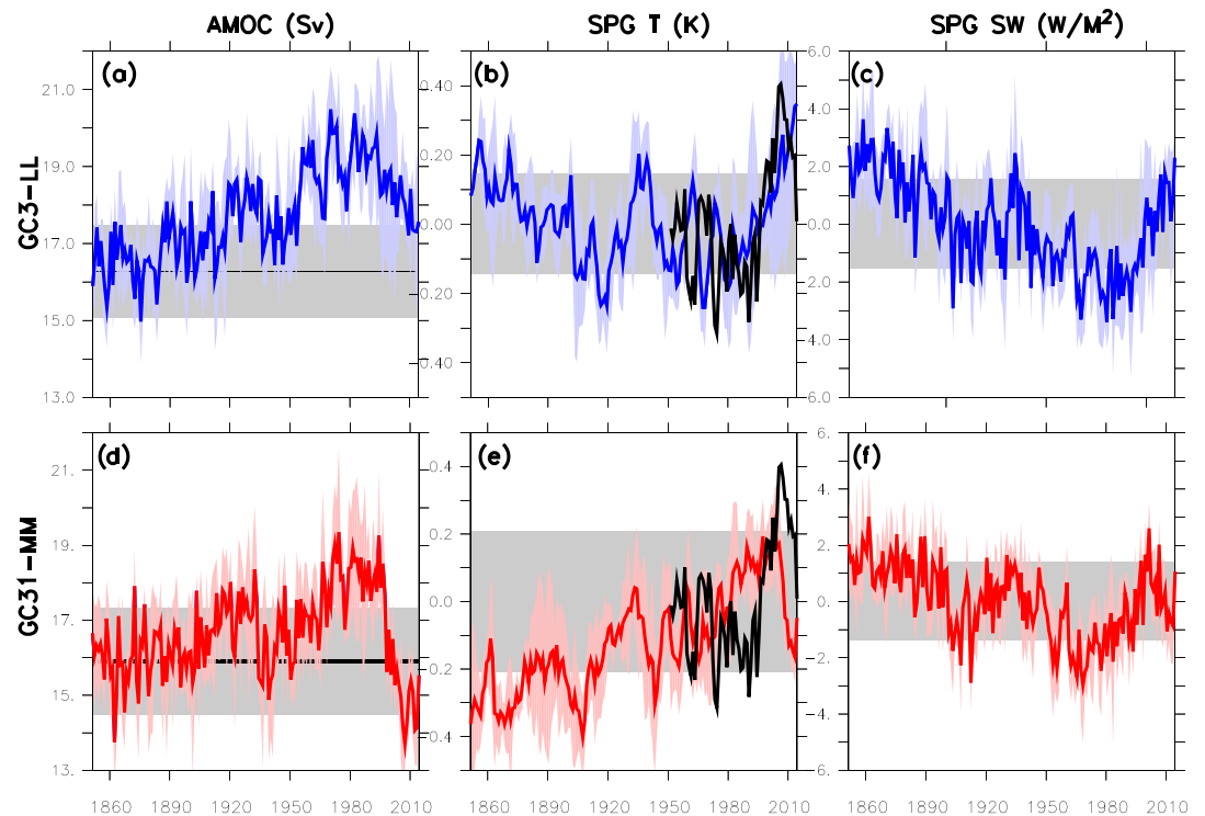
Figure 17. AMOC, subpolar heat content, and SW surface fluxes for GC31-LL (blue) and GC31-MM (red). (a) AMOC at 40°N (max of stream function—northward ocean velocity integrated from surface downward). Blue shading is 1 standard deviation of the ensemble spread. Black—mean of GC31-LL preindustrial (PI) control run (498 years) and shading is 1 standard deviation of the PI control. (b) GC31-LL ensemble mean ocean temperature anomaly (°C), mean over the Subpolar region (40:60°N, 0:60°W, 0–700 m). Shading as (a). Black: observations (EN4; Good et al., 2013). (c) GC31-LL Mean surface downward Shortwave flux ( W/m^2 ) into the ocean surface over the Subpolar Gyre region. Shading as (a). (d–f) As in (a)–(c) but for the GC31-MM historical experiment and the GC31-MM piControl experiment (378 years).
