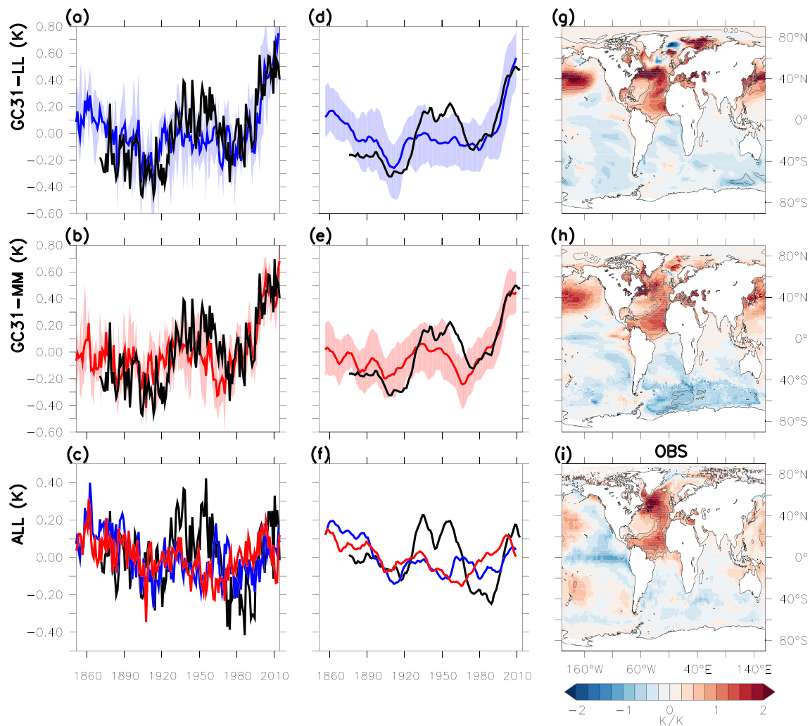
Figure 16. Time series and spatial patterns of AMV in model and observations. (a) Basin mean AMV (SST averaged over 7.5°–75°W, 0°–60°N) in GC31-LL using annual mean data (blue line: ensemble mean, shading: max/min across ensemble) compared with Observations (black: HadISST Rayner et al., 2003). All indices are anomalies with respect to their 1870–2014 mean (i.e., the observational period). (b) As in (a) but for GC31-MM (red). (c) AMV-GMT: ensemble mean AMV after the global (excluding Atlantic) mean temperature signal (GMT) was removed by linear regression (see text for details) (GC31-LL: blue, GC31-MM: red, obs: black). (d–f) As in (a)–(c) but indices have been smoothed with a 10-year running mean. (g) GC31-LL Ensemble mean SST-GMT regressed onto Ensemble mean AMV-GMT index. SST-GMT: SST after removing GMT by regression (see text). Shading is the coefficient of regression, contours the fraction of the variance explained (square of the correlation coefficient, contour interval: 0.2). (h) As in (g) but for GC31-MM. (i) As in (g) but for observed SSTs.
