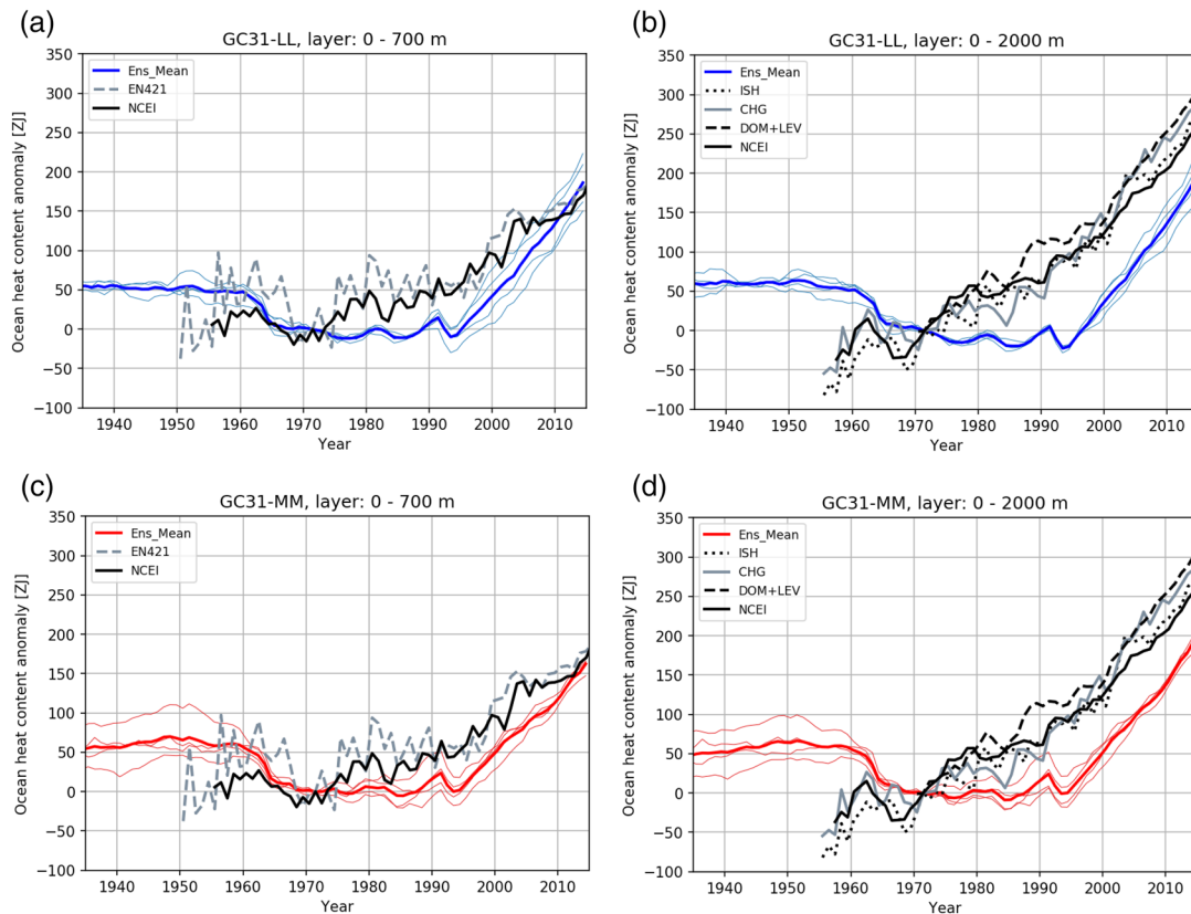
Figure 5. Time series of annual mean global ocean heat content anomaly for GC31-LL (a, b) and GC31-MM (c, d) in the 0- to 700-m layer (a,c) and the 0- to 2,000-m layer (b, d). Ensemble means in bold color (blue for GC31-LL, red for GC31-MM); individual ensemble members in thin colored lines; various observational products in thick gray and black lines. All time series normalized to the year 1971. In the 0- to 2,000-m panels the NCEI data are 5-year running means.
