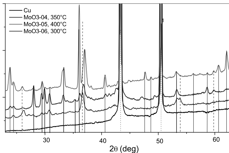
Figure 2. XRD spectra of \text{MoO}_3 films deposited at different temperatures and deposition times ( p\text{O}_2 = 0.1\text{--}0.2 mbar). Continuous lines highlight the \text{MoO}_3 phase peaks, whereas dash and dot lines identify the \text{MoO}_3 (or mixed \text{MoO}_3 + \text{MoO}_2 ) phase and the Cu substrate peaks, respectively.
