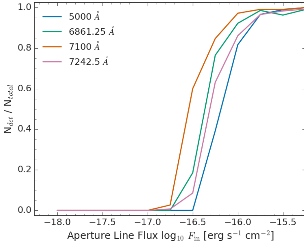
Figure 5.9: Recovery fraction detected/injected, from the insertion and detection of fake point sources for four different wavelengths within a single MUSE datacube. The detection process follows that used for the targeted observations.
