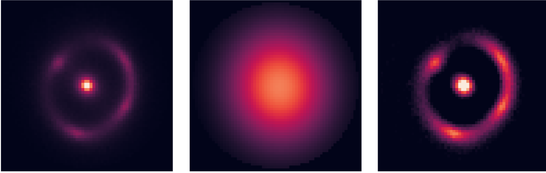
Figure 2.2: An example of phase one in the PYAUTOLENS pipeline, the initial light profile fitting. In the left panel, a simulated gravitational strong lens with a central lens galaxy at z = 0.5 , and a near complete Einstein ring for a background source at z = 1.0 . The second panel contains the initial simple fit for the light profile of the lens. In the right panel is the residual. At this stage the lens light residual is large, as the source was not masked.
