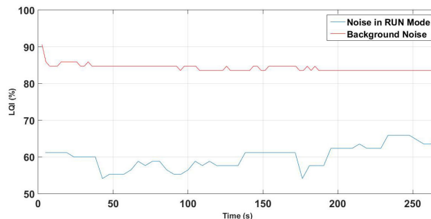
FIGURE 17. Difference in percentages between background noise with, and without the converter running.
