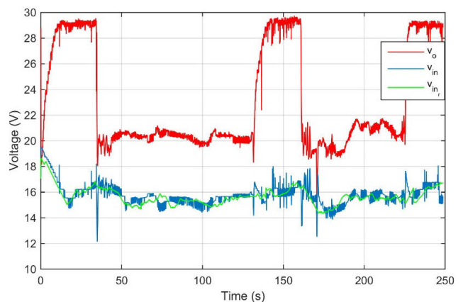
FIGURE 20. Reference voltage, DC/DC converter input and output voltage.
