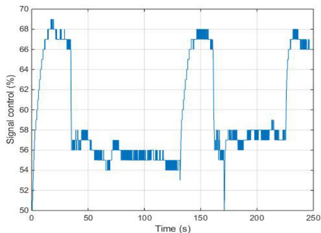
FIGURE 23. Control signal.
