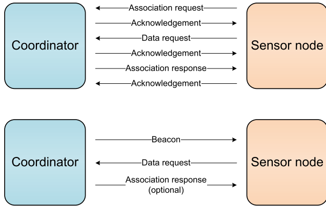
FIGURE 11. Association protocol for IEEE 802.15.4 beacon.
