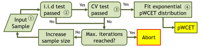
Fig. 8: Main steps in MBPTA-CV application.
