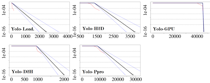
Fig. 13: pWCET estimates for YOLO stages.
