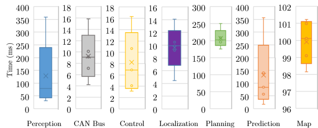
Fig. 1: Observed per-module execution time of Apollo
