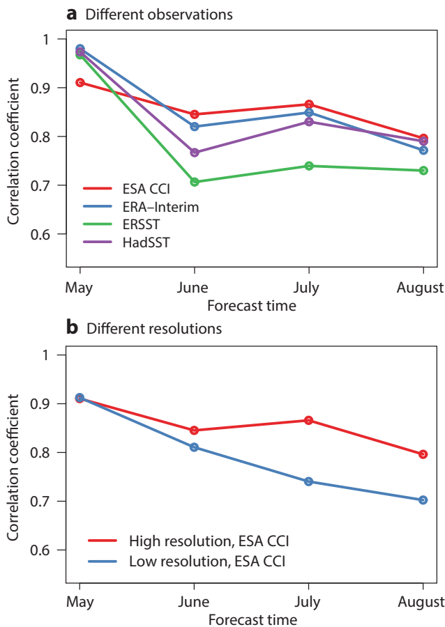
Figure 2 Correlation coefficient as a function of forecast time of ensemble-mean predictions of NINO3.4 sea-surface temperature performed with EC-Earth3.1 and initialised on 1 May using (a) the TL511-ORCA025 resolution configuration over the re-forecast period 1993 to 2009, for four different observational datasets, and (b) TL511-ORCA025 and TL255-ORCA1 re-forecasts verified against the ESA CCI dataset. All correlations are significant at the 5% confidence level and differences in the correlations in (b) are significant at the 1% confidence level.
