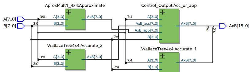
Figura 8. Circuit AM1_2.
