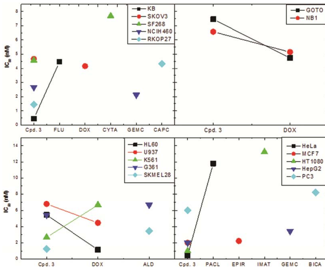
Fig. 1 — Effect of compound 3 on the viability of different tested cancer cell lines
