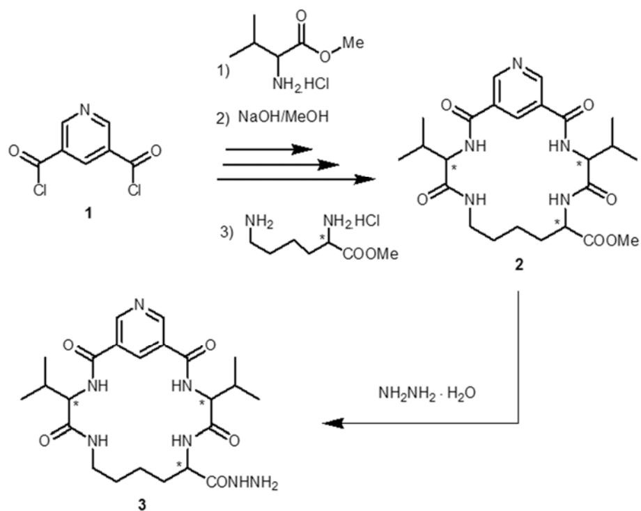
Scheme 1— Synthetic pathway for compound 3
