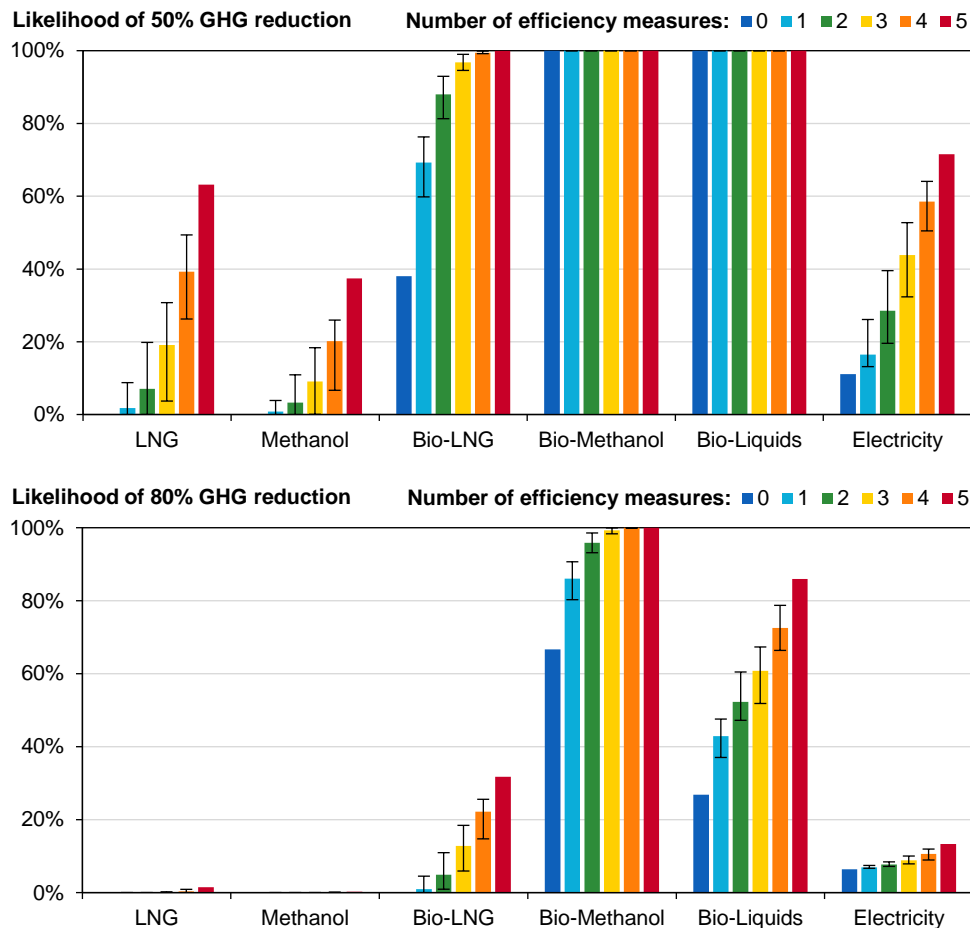
Figure 13. Probability of meeting the 50% GHG emission reduction target (top) and a stronger 80% target (bottom) via the use of alternative fuels alongside combinations of 5 different efficiency measures (renewable assisted propulsion, slow steaming, hydrodynamics, engine design and ship design).
