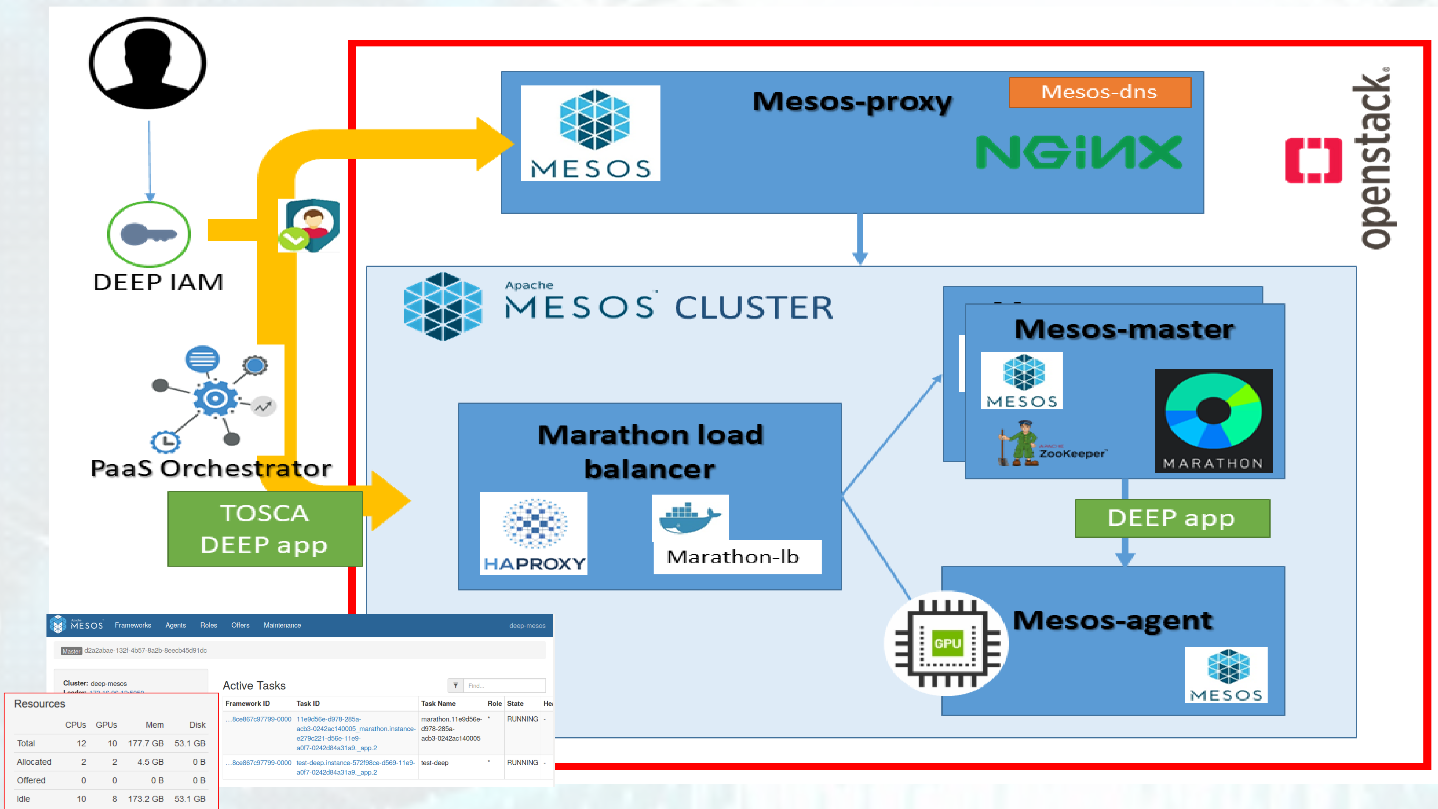
Figure 1. Integration of Mesos + Marathon in DEEP using GPUs
