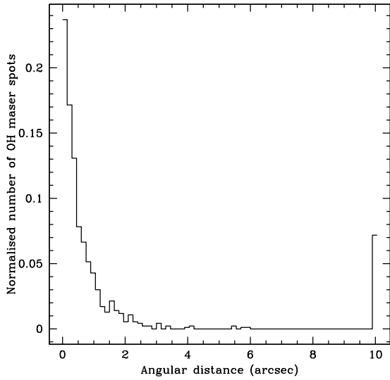
Fig. 7.— Distribution of the angular distance to the nearest neighbour for each maser spot. This figure is cut off at 10'' where a higher number of unrelated nearby sources start to show.
