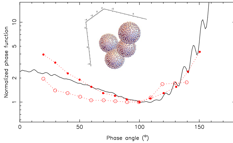
Fig. 2.— OSIRIS phase functions (red solid circles for MTP020/071 and red open circles for MTP025/092) compared with MSTM calculations (solid black line) for peppered sphere clusters such as that shown on the inset. XYZ labels on the inset are given in \mu\text{m} . All phase functions are normalized to unity at a phase angle of 100.
