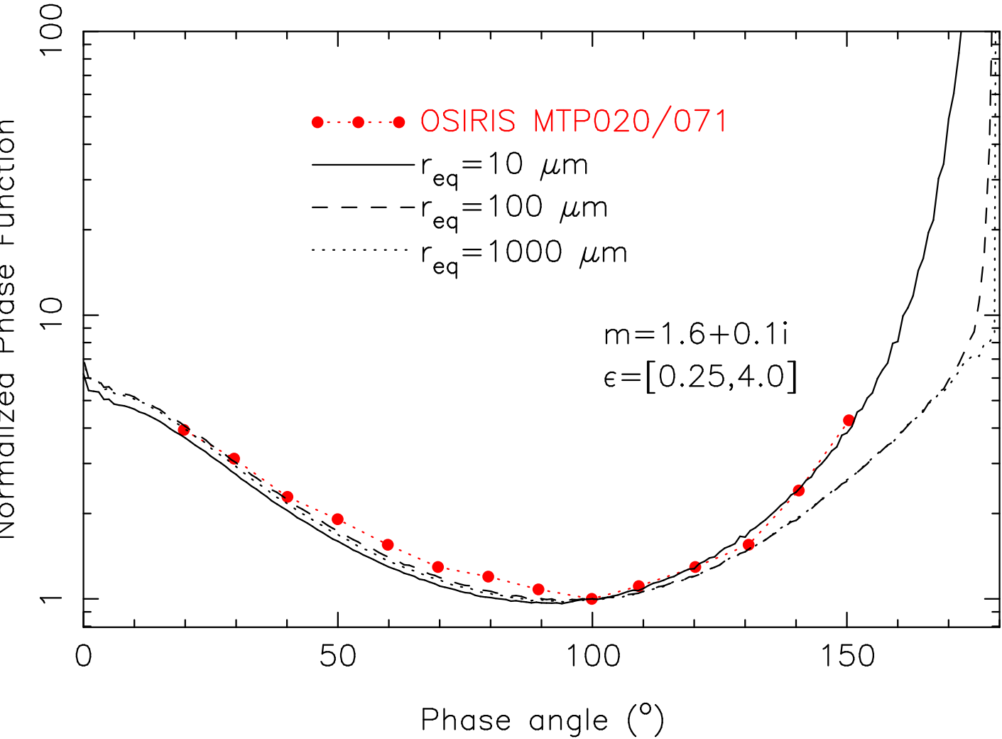
Fig. 5.— OSIRIS phase function measurements for MTP020/071 (solid red circles) compared to geometric optics simulations for three distributions of spheroids with uniform axes ratio in the \epsilon = [0.25, 4.0] interval, and having equivalent spherical radii of 10 \mu\text{m} (black solid line), 100 \mu\text{m} (black dashed line), and 1000 \mu\text{m} (black dotted line). All phase functions are normalized to unity at 100^\circ of phase angle. As in all the simulations in this work, the refractive index is set to m = 1.6 + 0.1i .
